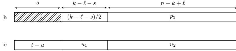
Fig. 5.2. The form of the parity-checks produced by this method [3], vs. the bet made on the error. The hatched rectangle of size s for \mathbf{h} indicates that the weight is arbitrary on this part.
