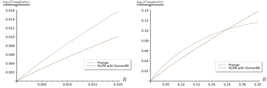
Fig. 4.2. The complexity of the RLPN-decoder for very small rates vs. the simplest information set decoder, namely the ISD Prange decoder [24]. For small R , there is not much difference between the ISD Prange decoder and much more evolved decoders like [3, 20, 5, 6]. The RLPN-decoder with the very simple [10] technique performs much better for small rates than ISD decoders. It is only outperformed by the Prange decoder for rates above 0.25 approximately.
