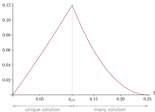
Fig. 1.1. Complexity exponent \alpha of the Prange ISD algorithm [24] as a function of the error ratio \tau \triangleq \frac{t}{n} at rate R = \frac{1}{2} . The peak corresponds to the normalized Gilbert-Varshamov distance \delta_{\text{GV}} = h^{-1}(1-R) .
