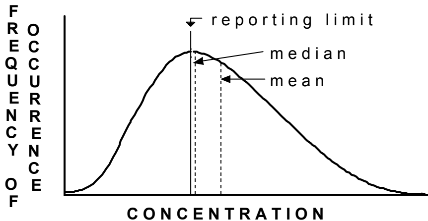
Figure 13.2. Distributional (MLE) method for computing summary statistics.
