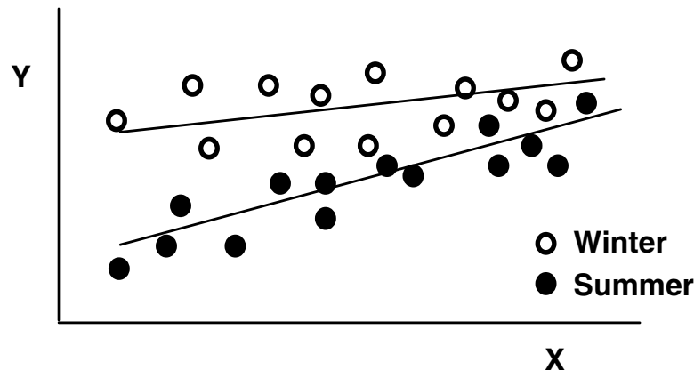
Figure 11.5 Regression lines differing in slope and intercept for data from two seasons
