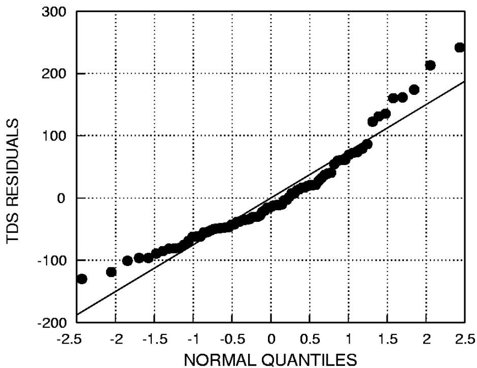
Figure 9.13 Probability plot of the TDS regression residuals
