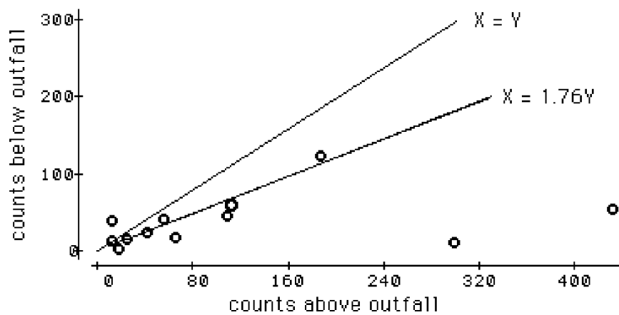
Figure 6.7 Mayfly data with multiplicative relationship x = y \cdot 1.76 .
