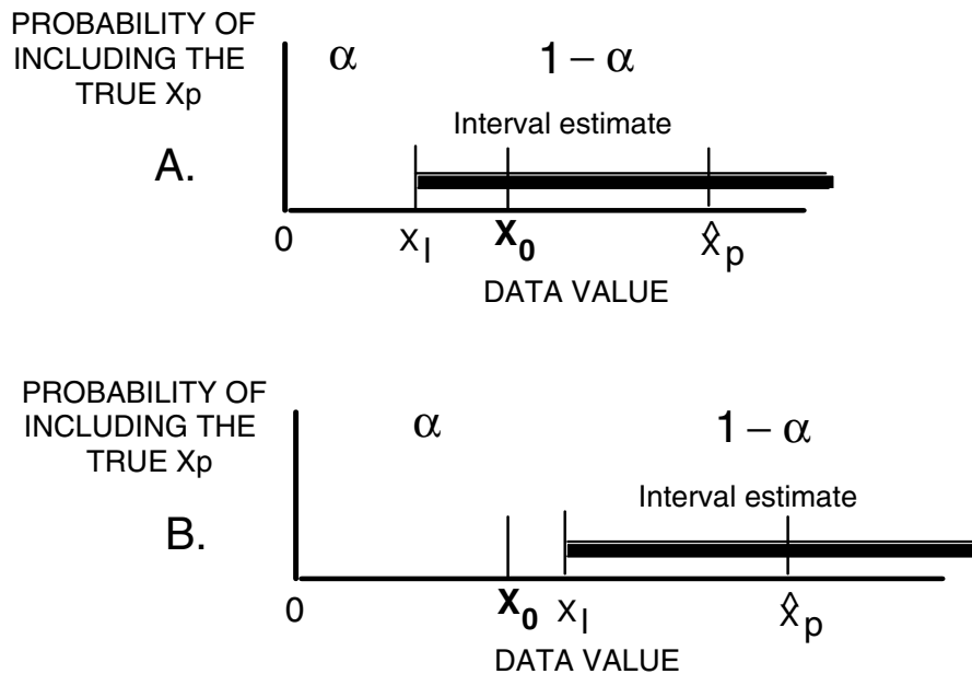
Figure 3.10 One-sided interval estimate as a test for whether percentile X_p > X_0 . A. X_0 inside interval estimate: X_p not significantly greater than X_0 . B. X_0 below interval estimate: X_p significantly greater than X_0 .
