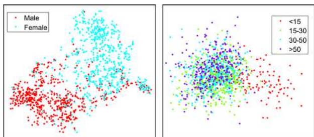
Fig. 22 Embedding of 1212 Headspace per-subject shape vectors into a 2D space, using gender labels (left, 606 males and 606 females) and age labels (right). We use t-Distributed Stochastic Neighbor Embedding (Van Der Maaten 2014)
