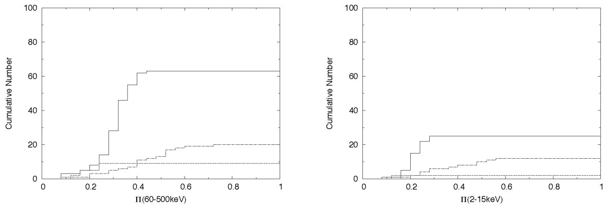
FIGURE 1. The cumulative distribution of \Pi that can be measured by GRAPE ( left ) and LEP ( right ) in the SO ( solid ), SR ( dashed ), and CD ( dot-dashed ) models in which the number of detectable bursts is 200. The adopted parameters are \gamma = 100, q_1 = 0.5, q_2 = -2.0, \alpha = -0.2, \beta = 1.2 , and T = 20 s.
