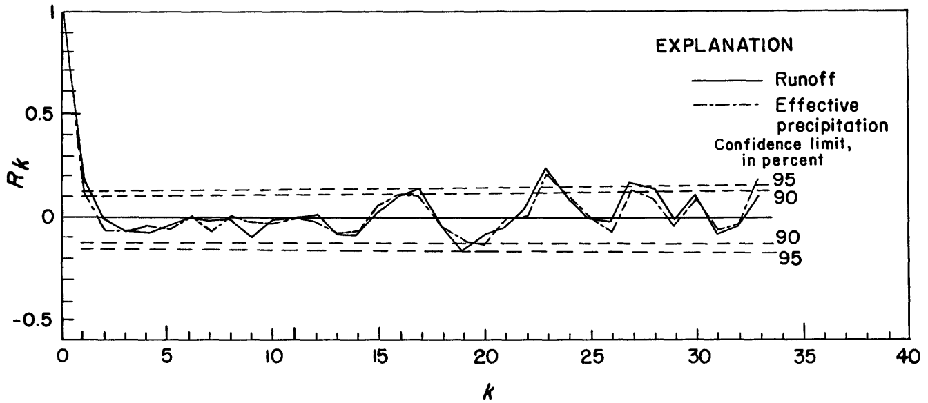
FIGURE 3.—Correlograms of runoff and effective precipitation for the Nemunas River at Smalininkai, Lithuania.
