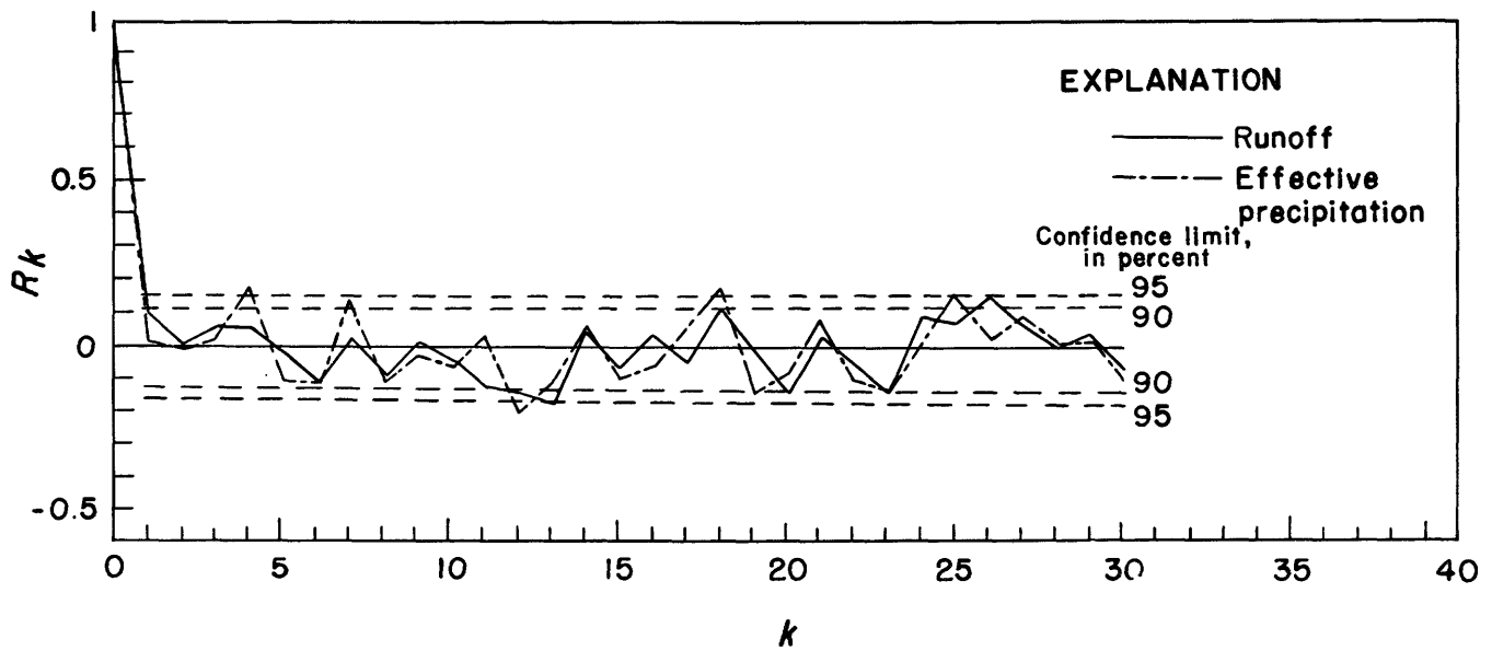
FIGURE 4.—Correlograms of runoff and effective precipitation for the Danube River at Orshava, Rumania.
