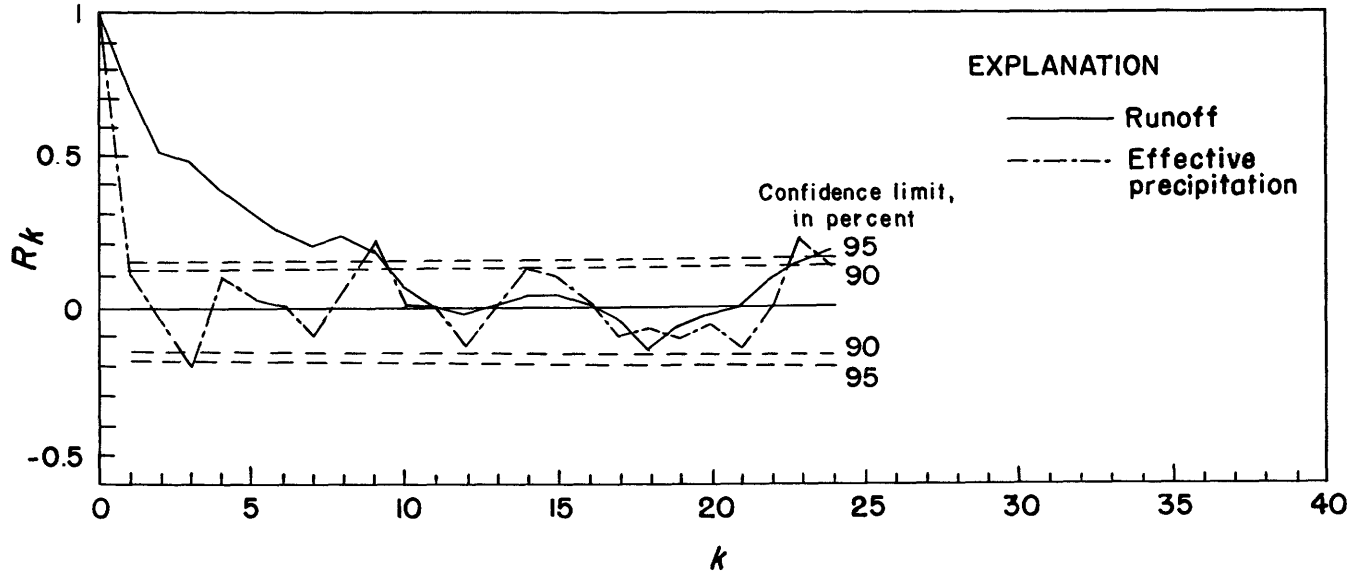
FIGURE 1.—Correlograms of runoff and effective precipitation for the St. Lawrence River at Ogdensburg, N.Y.
