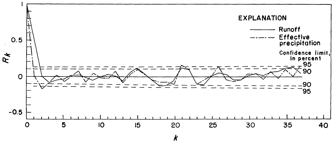
FIGURE 2.—Correlograms of runoff and effective precipitation for the Göta River at Sjötorp-Vänernborg, Sweden.
