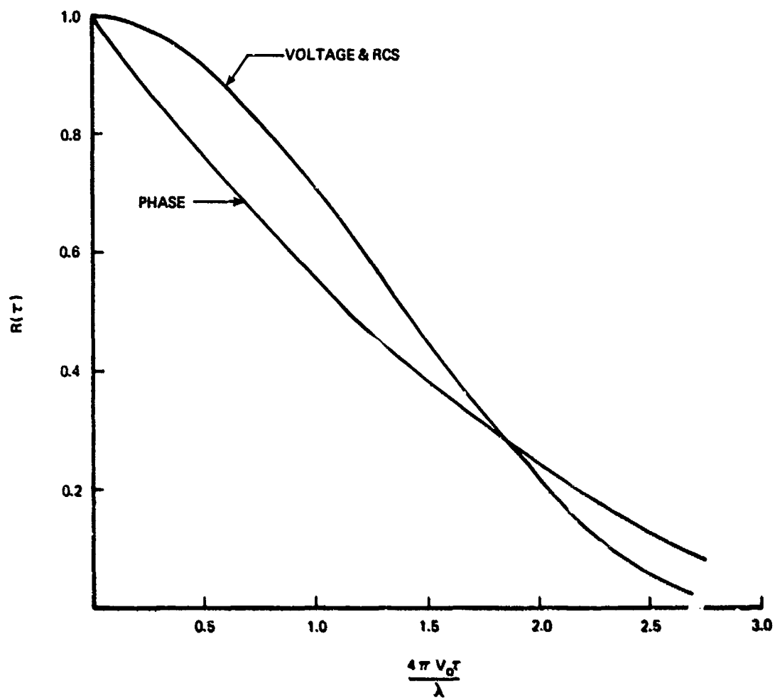
Figure 6. Voltage, RCS and Phase Auto-covariance Functions for Constant Speed Distribution
