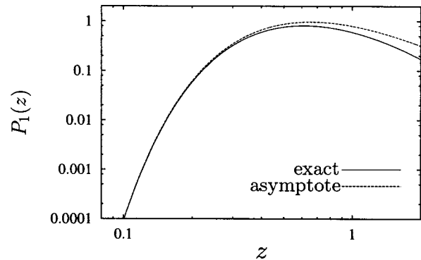
FIG. 3. The PDF P_1(z) from Eq. (10) with N=100 and its small- z asymptote as given by Eq. (17).
