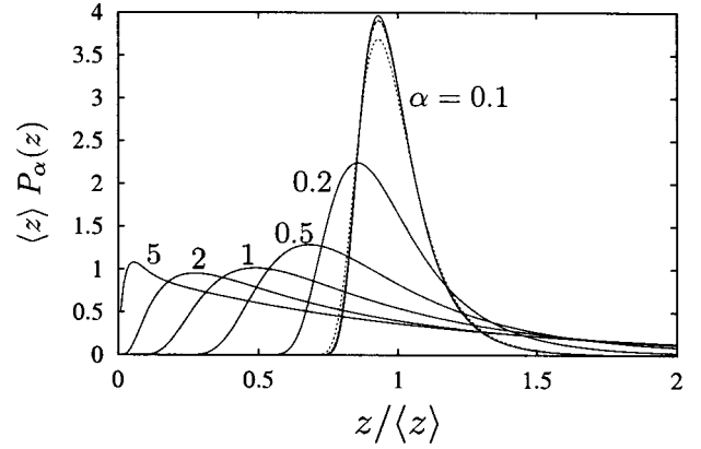
FIG. 4. Distribution functions for d=1 and various \alpha 's. We rescaled z by its mean \langle z \rangle to get a variable of unit average. For \alpha=0.1 we show the sequence of approximants with N=10^5, 10^6, 10^7 peaks moving upwards with increasing N , to demonstrate slow convergence.
