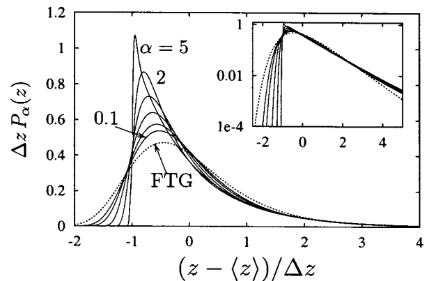
FIG. 5. The PDF with the same \alpha 's as in Fig. 4, but z is now shifted by its mean \langle z \rangle and rescaled by its standard deviation \Delta z to produce a variable of zero average and unit deviation. For \alpha=0.1 only the curve with the largest N is shown. The peaks decrease with \alpha . The PDFs tend to the FTG function (dashed line). The semilogarithmic inset magnifies the small- P regions.
