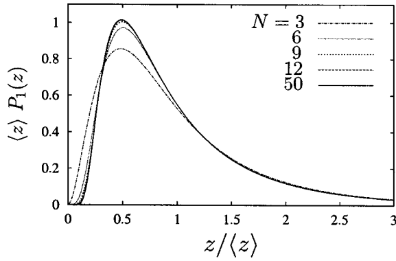
FIG. 1. Distribution functions for the \alpha=1 case evaluated numerically according to Eq. (10) for various N 's, each function scaled to unit average. The convergence is apparently fast for practical purposes.
