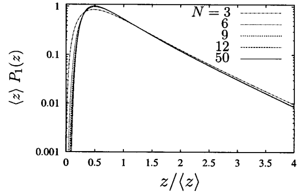
FIG. 2. The same as Fig. 1 on a semilogarithmic scale so as to better display the regions where P_1(z) is small.
