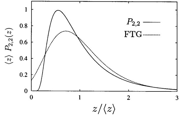
FIG. 6. Distribution function for the maximum Fourier intensity statistics for d=\alpha=2 and the FTG function scaled to unit mean and the same variance.
