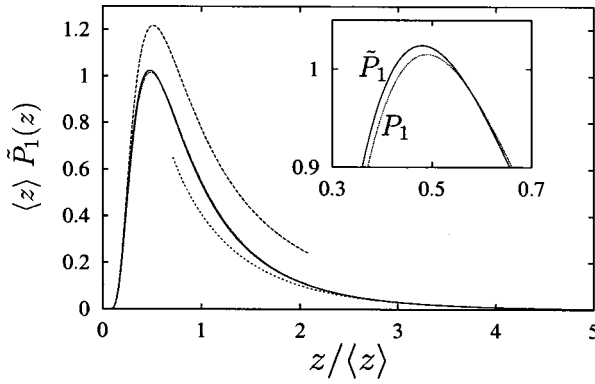
FIG. 7. The extreme value PDF \tilde{P}_1(z) , computed from Eq. (45) with \alpha=d=1 (full line), the asymptotes for small z from Eq. (47) (dashed), and for large z (48) (short dashed). For comparison the maximal intensity PDF P_1(z) from Fig. 1 is also shown (dotted); the two PDFs are very close, but distinct, as can be observed also near the maximum (see inset).
