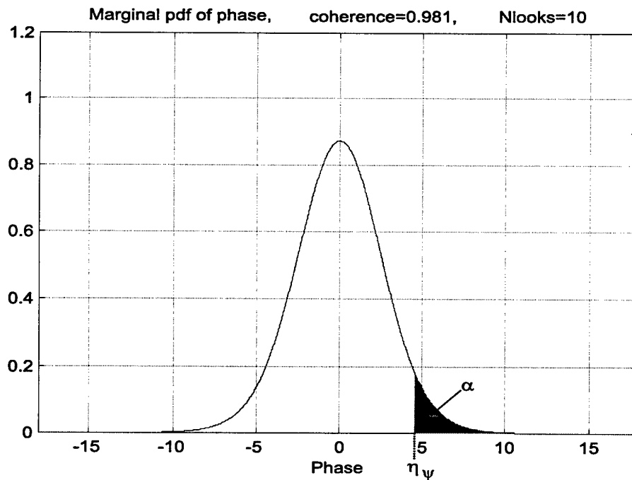
Figure 27 : Phase threshold for the moving target detector depending on the given false alarm probability.
