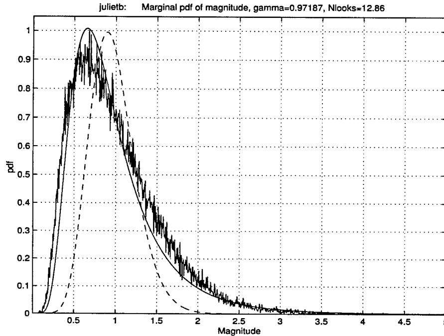
Figure 30 : Histogram of the interferometric magnitude for the highway area along with the p-distribution (solid) and the original magnitude pdf (dashed).
