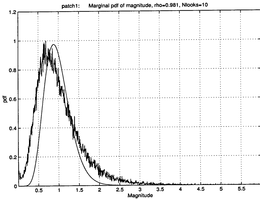
Figure 10 : Ten-look theoretical and empirical normalized magnitude probability density function for patch one.
