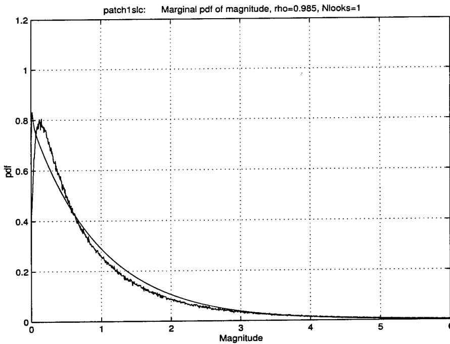
Figure 9 : One-look theoretical and empirical normalized magnitude probability density function for patch one.
