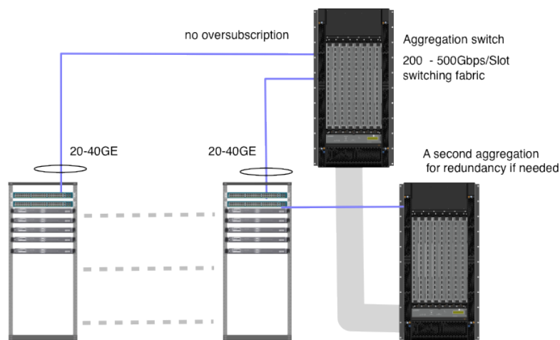
Figure 3. Connecting ToR access switches at LHC Tier1s
