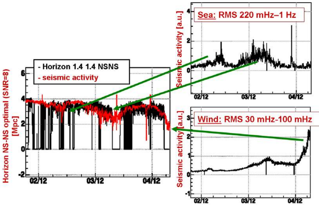
Figure 4. In the upper-right plot the seismic activity due to sea is reported, estimating the RMS in the range 0.221\text{Hz} . In the lower-right plot the seismic activity due to wind is reported, estimating the RMS in the range 0.030.1\text{Hz} . In the left plot the horizon estimated with the detector sensitivity and with the empirical formula is reported.
