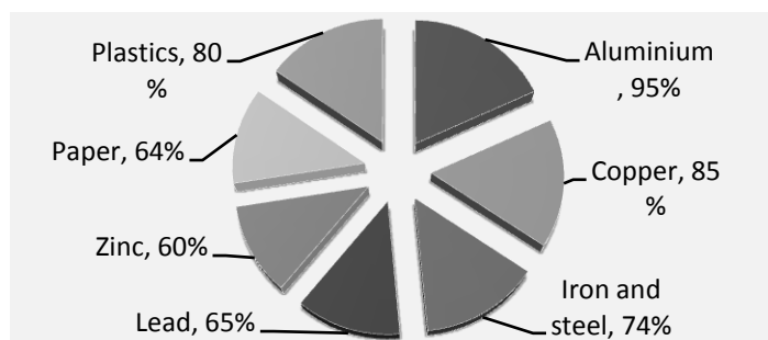
Figure 7 Energy saving %age by recycled material [Cui, 2003]
