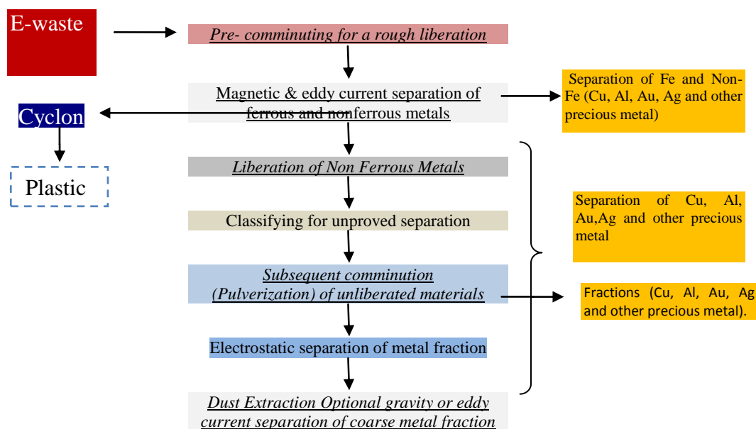
Fig: 11 Process Flow of Non-Ferrous Based E-wastes Treatment [MoEF, Guidelines, 2008].
