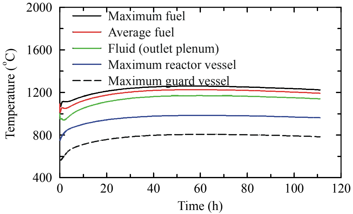
Fig. 6.8. Thermal performance following a LOFC.
