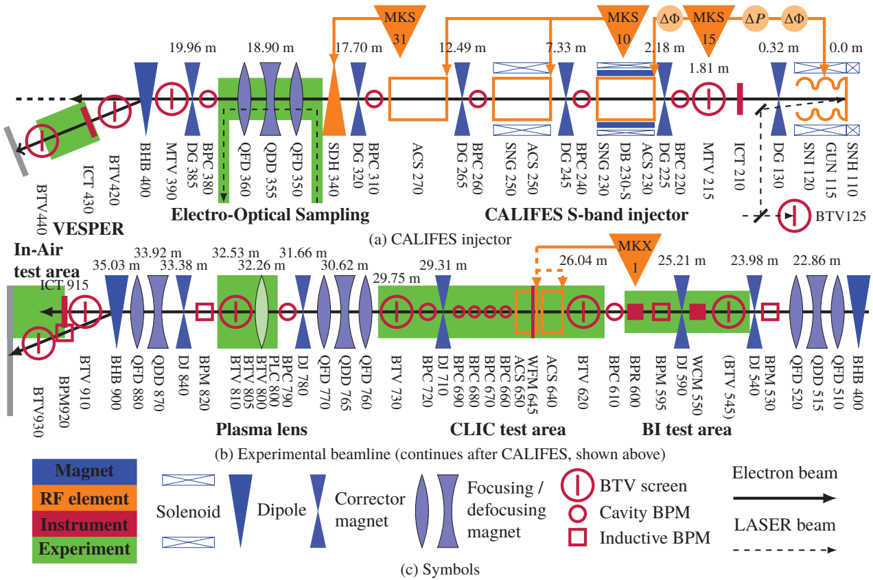
Figure 1: Overview of the elements directly interacting with the beam at CLEAR beamline, and the location of the experimental stations as of April 2019. Element positions indicate the middle of each element, rounded to the nearest cm.
