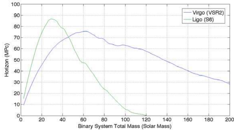
FIGURE 4. VSR2 Virgo horizon compared to Ligo horizon.
