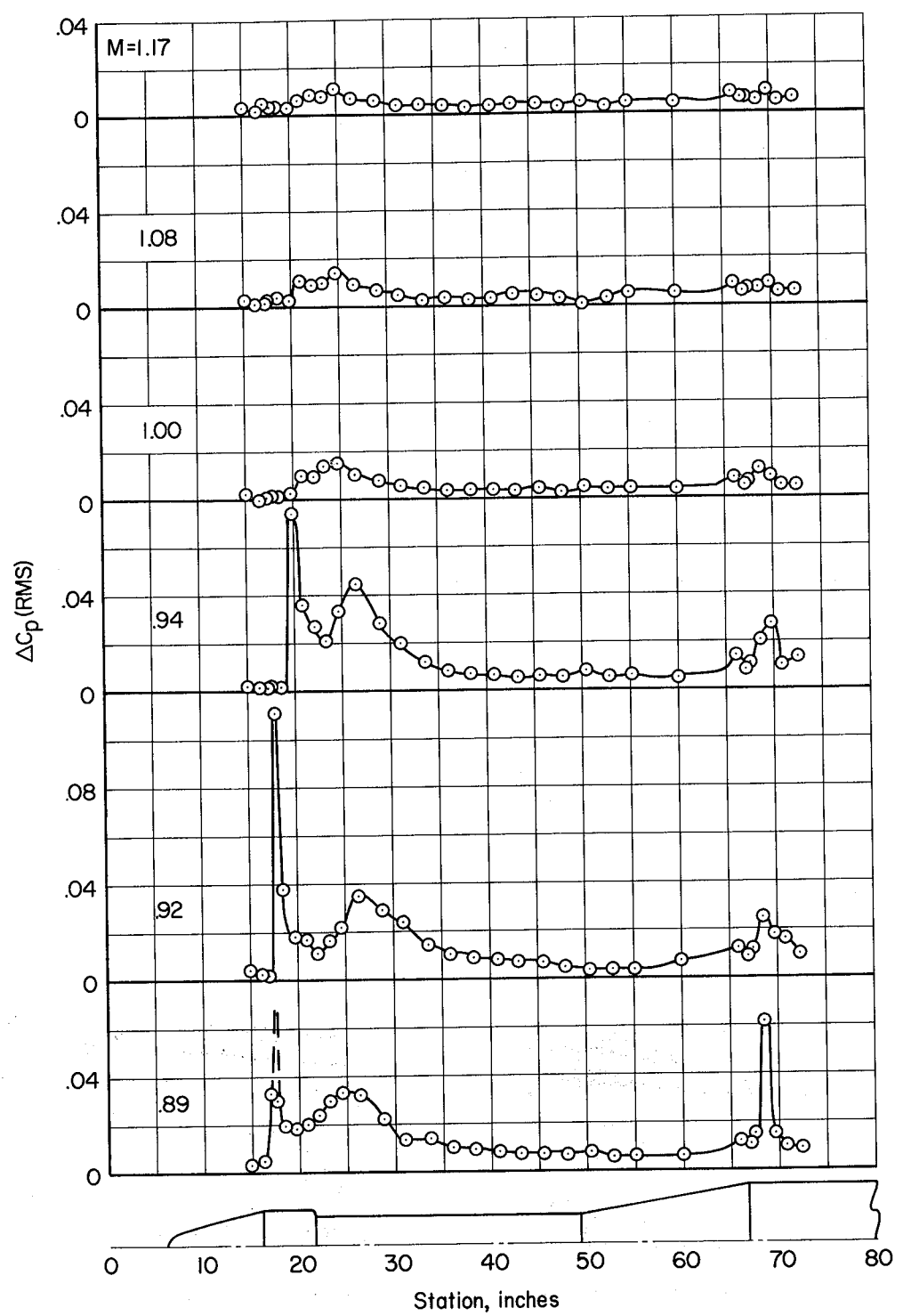
(d) \alpha = 8^\circ - Concluded.
