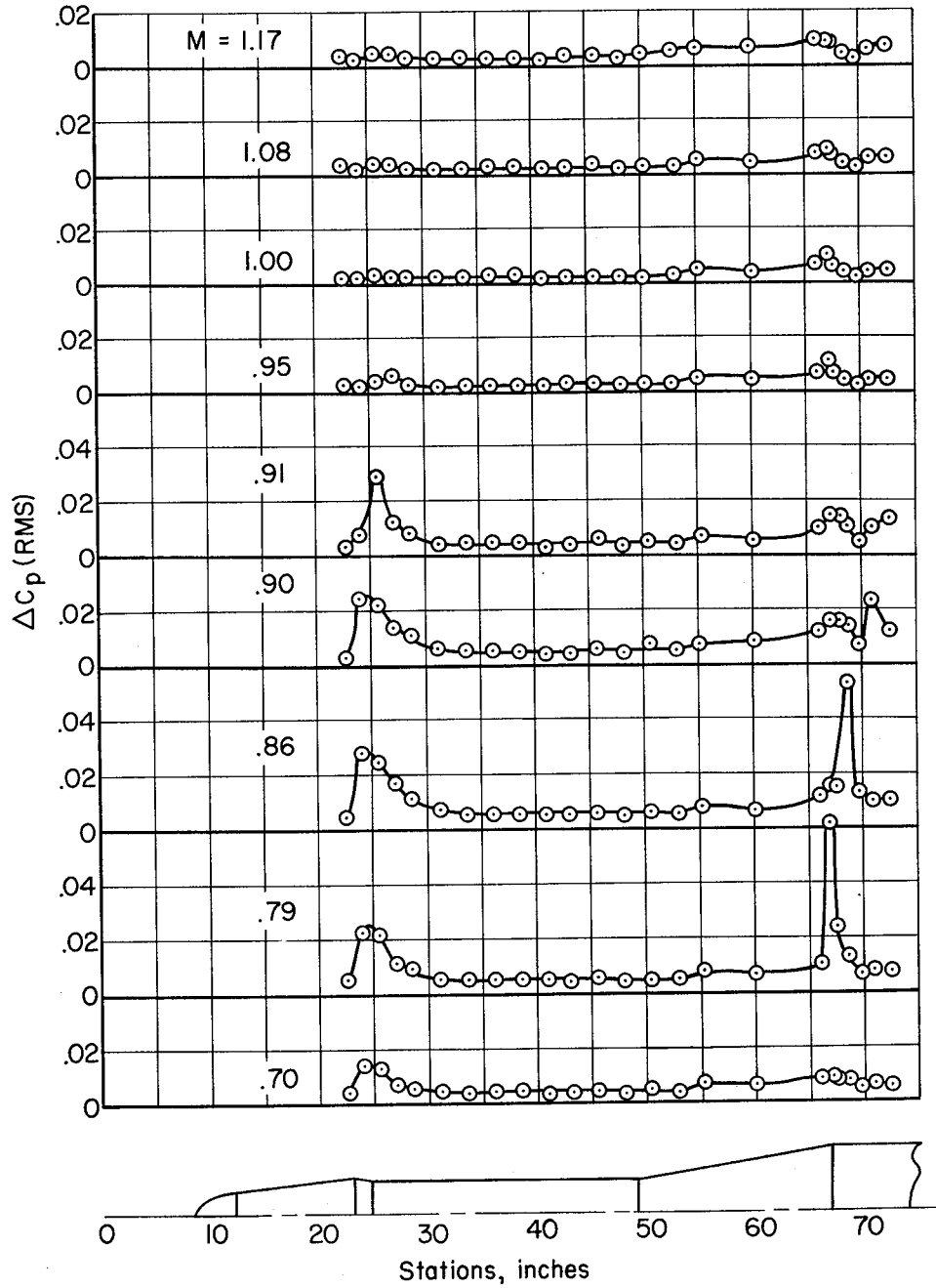
Figure 7.- Longitudinal distribution of the pressure fluctuations on model 12.
