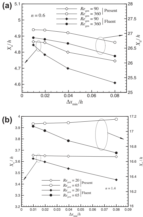
Fig. 3. Dependence of vortex characteristics ( X_a and X_d in case of symmetric flow and asymmetric flow with a third eddy, respectively) on the smallest grid size ( \Delta x_{\min}/h ) corresponding to different meshes obtained with our code and Fluent: (a) n = 0.6 and (b) n = 1.4 .
