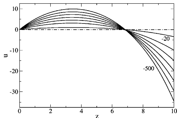
FIG. 16. Asymptotic profiles of the horizontal fluid velocity u across the layer at x=x_{|u|=|u|_{\text{max}}} for decreasing negative Marangoni numbers between -20 and -500 with an interval of 80 between two successive curves. The dot-dashed curve corresponds to M=0 when there is no convection.
