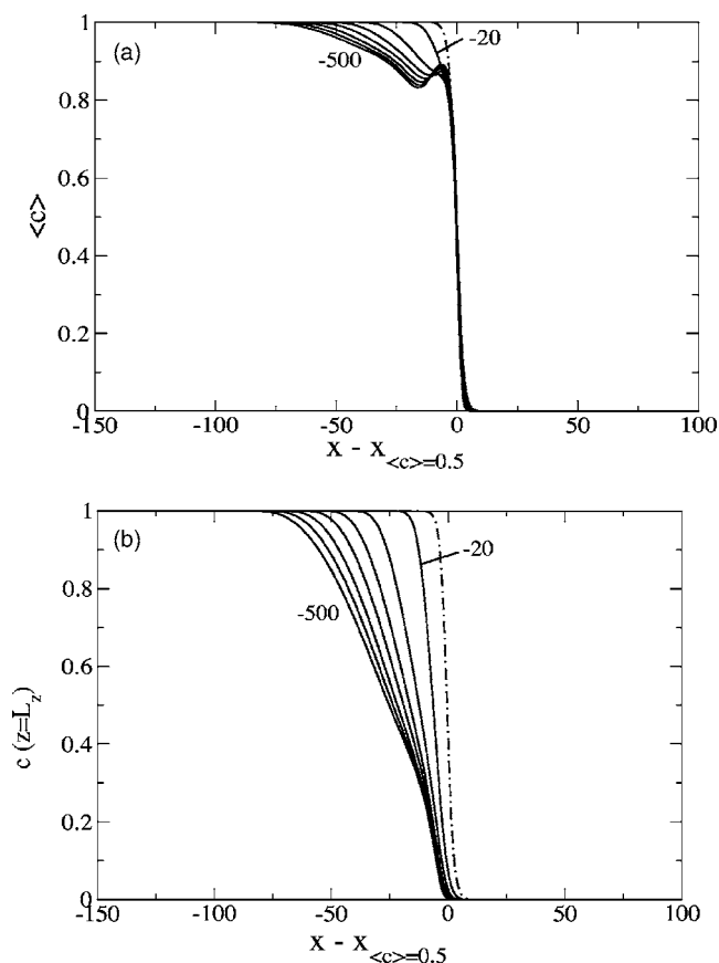
FIG. 15. Asymptotic profiles of (a) the averaged concentration \langle c \rangle and of (b) the surface concentration, represented in the comoving frame for decreasing negative Marangoni numbers between -20 and -500 with an interval of 80 between two successive curves. The dot-dashed curve corresponds to the RD profile.
