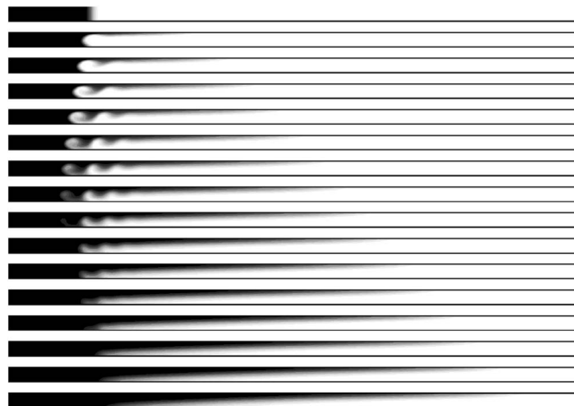
FIG. 4. Transient oscillating deformation of a chemical front due to chemically induced Marangoni convection at high Marangoni number ( M=1000 ). The dynamics is shown from top to bottom from t=0 up to t=15 with a time interval of \Delta t=1 . The aspect ratio between L_x=350 and L_z=10 is preserved.
