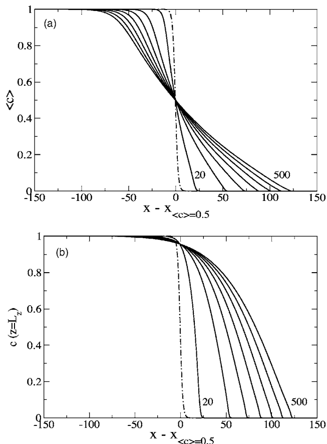
FIG. 9. Asymptotic profiles of (a) the averaged concentration \langle c \rangle and of (b) the surface concentration represented in the coming frame for increasing positive Marangoni numbers between 20 and 500 with an interval of 80 between two successive curves. The dot-dashed curve corresponds to the RD profile.
