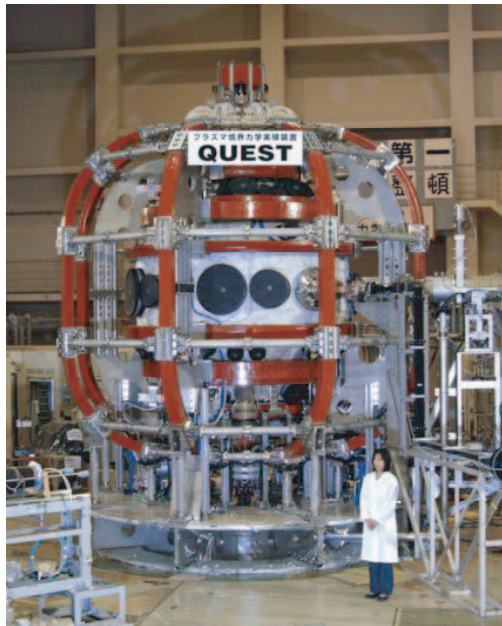
Fig. 2 The vacuum vessel and TF, PF coils of QUEST
