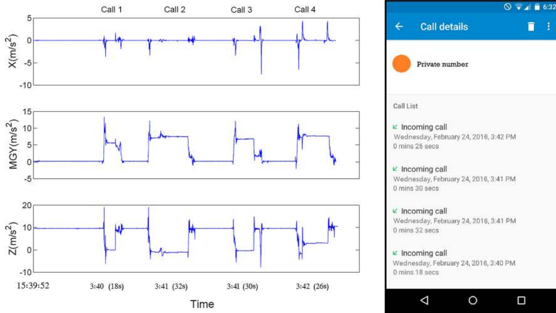
Fig. 2 Left Three dimensions ( x , y , and z ) of acceleration data including gravity (from the motion sensor). The start time, duration, and end time of four phone calls are easily recognizable from these measurements. Right The screenshot of the call history of the phone during the experiment
