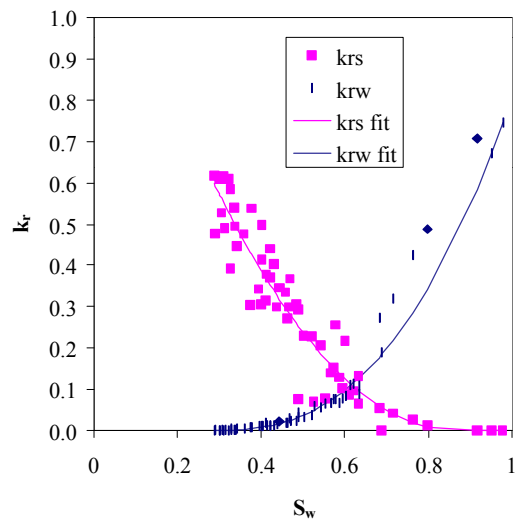
Figure 11: Fit to Mahiya (1999) results.
