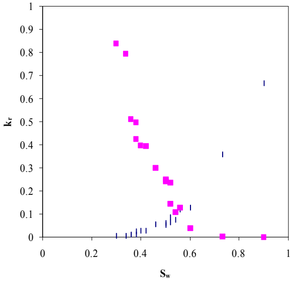
Figure 4: Experimental results from Satik (1998).
