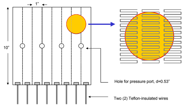
Figure 7: Schematic of flexible heaters.
