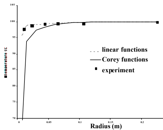
Figure 13: Fracture flow (temperature vs. radius) results from Wang and Horne (1999). Match using X-curves shown as dashed line, match using Corey curves shown as solid line.
