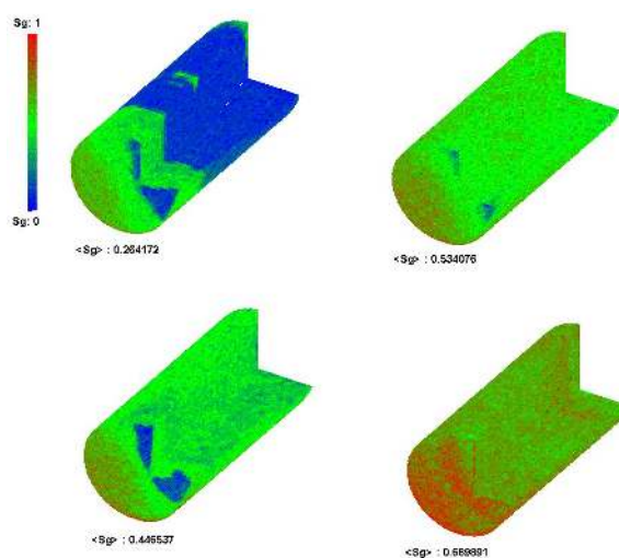
Figure 2: Steam distributions measured by X-ray CT, from Satik (1998).
