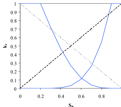
Figure 1: Corey (solid lines) and linear (dashed lines) relative permeability curves.
