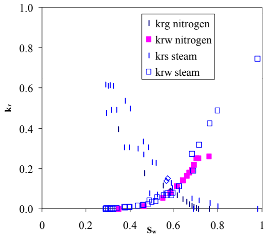
Figure 10: Comparison between steam-water (open symbols) and nitrogen-water imbibition (closed symbols) relative permeabilities on the same rock core.
