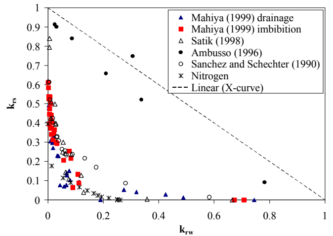
Figure 9: Comparison of results, k_{rs} vs. k_{rw} .
