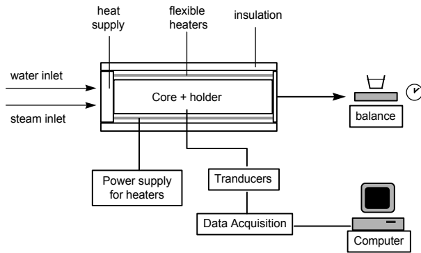
Figure 5: Experimental apparatus for the flow-through experiment using heat guards.
