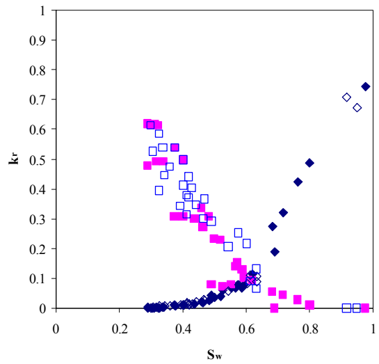
Figure 8: Experimental results from Mahiya (1999) adiabatic experiment. Closed symbols, drainage curves; open symbols, imbibition curves.
