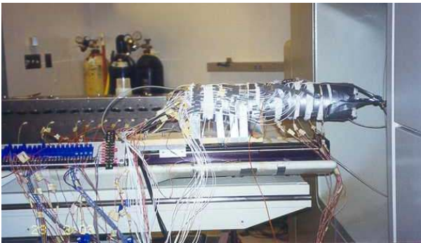
Figure 5: Experimental apparatus for the flow-through experiment using heat guards.
