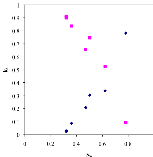
Figure 3: Experimental results from Ambusso (1996).
