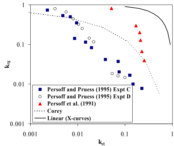
Figure 12: Some measurements of air-water relative permeabilities in rough-walled fractures.
