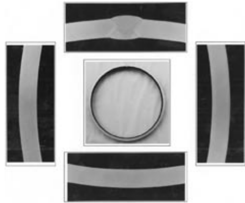
Fig. 13 Cross sections of the MARINE-COP after 3 years of service as a cargo oil tank in the BENETIA
