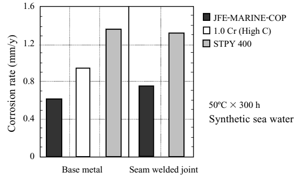
Fig. 12 Corrosion rate of JFE-MARINE-COP in synthetic sea water in comparison with those of 1% Cr, high C steel and STPY 400
