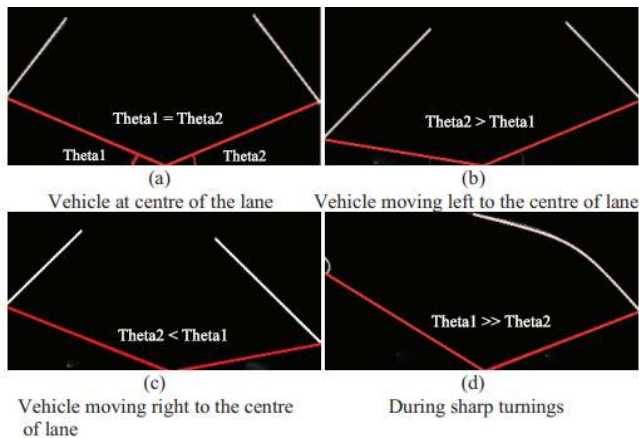
FIGURE 7: Cases of angular aberration from center of the road [83]
