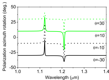
Fig. 6. (Color online) Rotation angle \delta between the principal axis of the polarization for the transmitted wave and the x direction with different incident polarizations \theta .
