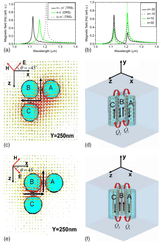
Fig. 2. (Color online) (a) Local magnetic field amplitude |H_z| detected between rods A and B for the TRS (black solid curve for \theta=-45^\circ and black dotted curve for \theta=45^\circ ) and DRS [green (gray) solid curve for \theta=0^\circ ]. (b) Magnetic field amplitude |H_z| calculated between rods A and B of the TRS for incident polarizations \theta=-30^\circ, -10^\circ, 10^\circ, 30^\circ . Local magnetic field vector profiles and current distributions (c)–(d) for the |\alpha\rangle mode at \lambda_\alpha=1.122 \mu\text{m} with \theta=-45^\circ and (e)–(f) for |\beta\rangle mode at \lambda_\beta=1.211 \mu\text{m} with \theta=45^\circ .
