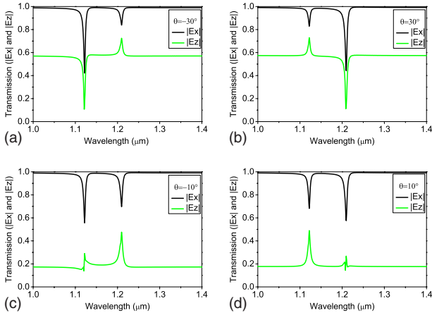
Fig. 7. (Color online) Retrieved amplitudes of the electric field components |E_x| and |E_z| by coordinate transformation theory. The chosen incident polarization angles from (a) to (d) are \theta = -30^\circ, 30^\circ, -10^\circ, 10^\circ .
