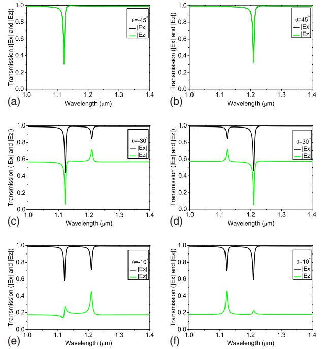
Fig. 3. (Color online) Amplitudes of the electric field components |E_x| and |E_z| when the plane wave passes through the metamaterial consisting of TRSs. The chosen incident polarization angles from (a) to (f) are \theta = -45^\circ, 45^\circ, -30^\circ, 30^\circ, -10^\circ, 10^\circ .
