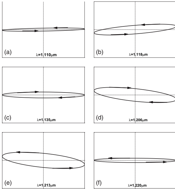
Fig. 5. Polarization patterns of the transmitted waves obtained at different wavelengths for the incident case \theta=0^\circ . The arrows in the figures indicate the rotation directions of the transmission waves.
