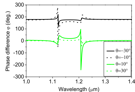
Fig. 4. (Color online) Phase difference between the two transmission electric components.
