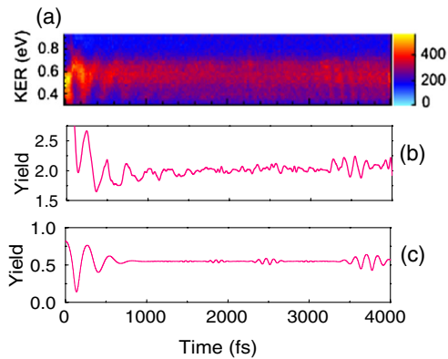
FIG. 4 (color online). (a) Measured time-dependent KER spectrum as in Fig. 3(a), but for an increased pump-pulse peak intensity of 9 \times 10^{14} W/cm 2 and an extended delay range. (b) Dissociation yield obtained by integration over the KER range in (a). (c) The calculated dissociation yield for the same KER range.
