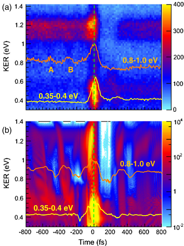
FIG. 3 (color online). (a) Measured \text{Ar}_2(1, 0) KER spectrum as a function of the pump-probe time delay for 60 fs laser pulses with a peak intensity of 10^{14} W/cm ^2 . (b) Corresponding calculated KER spectrum. The green dashed vertical line indicates zero time delay. The orange and yellow curves labeled with 0.8–1.0 eV and 0.35–0.4 eV are partial fragment yields obtained by integrating the spectra in (a) and (b) over the KER ranges from 0.8 to 1.0 eV and 0.35 to 0.4 eV, respectively.
