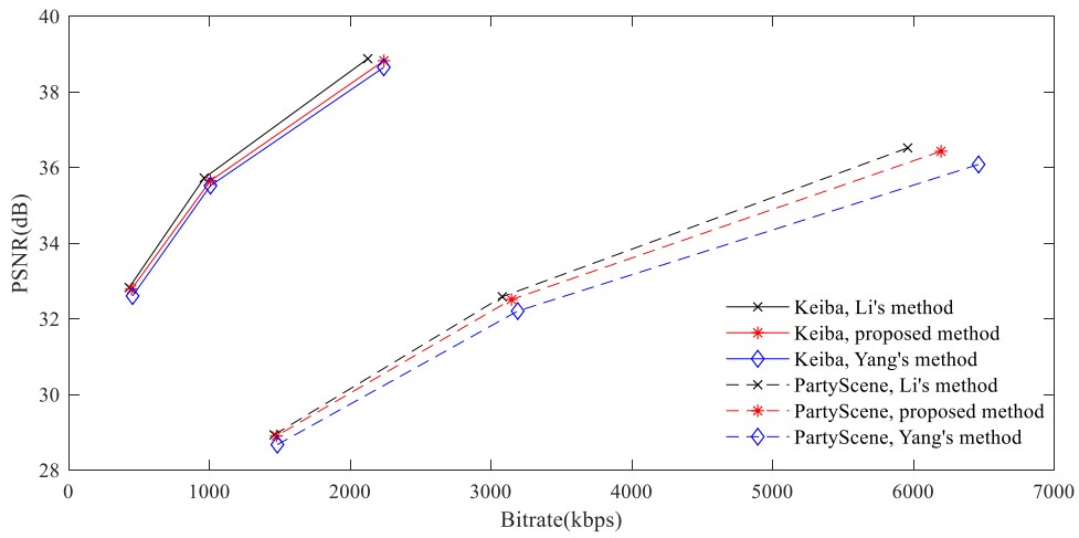
Fig. 10 Comparison of RD with Li's method and Yang's method for sequences Keiba and PartyScene
