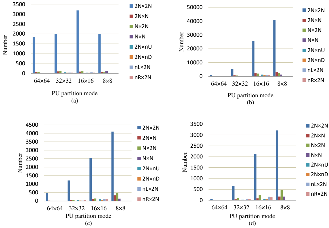
Fig. 3 Distribution of PU partition modes for videos with different resolutions (a) BasketballDrive_1920×1080. (b) PeopleOnStreet_2560×1600. (c) Chinaspeed_1024×768. (d) Race Horses_832×480.
