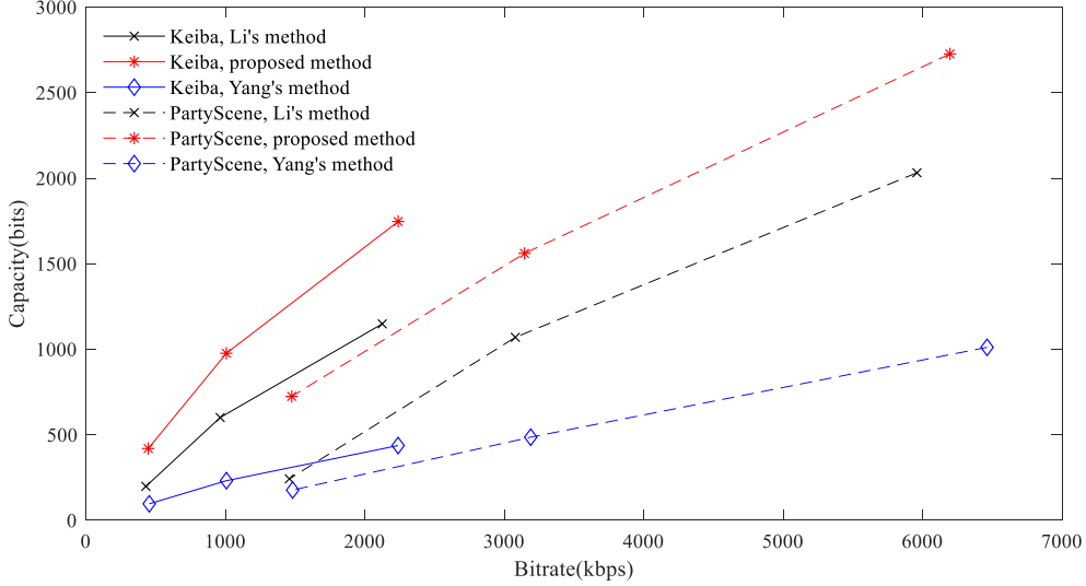
Fig. 8 Comparison of RC with Li's method and Yang's method for sequences Keiba and PartyScene
