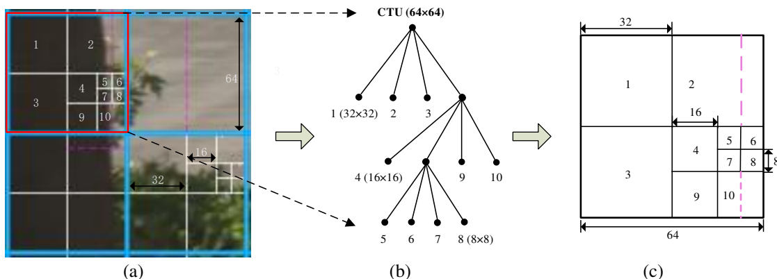
Fig. 1 Example of quadtree partition of CTU into CUs and PUs. (a) CTU partition. (b) CU partition quadtree. (c) PU partition.
