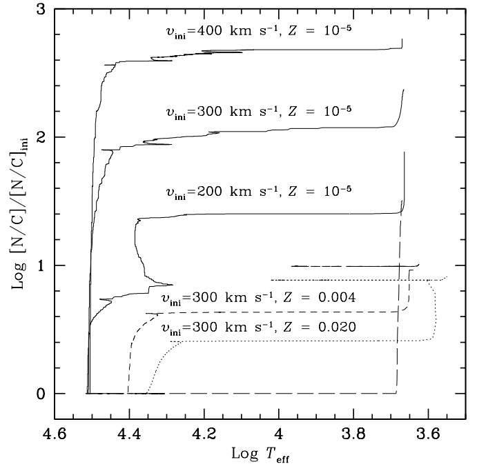
Fig. 12. Evolution as a function of \log T_{\text{eff}} of the abundance ratio N/C where N and C are the surface abundances of nitrogen and carbon respectively. The abundance ratios are normalized to their initial values. The tracks are for 9 M_{\odot} for different values of the metallicity, Z , and rotation. The long-dashed line, at the bottom, corresponds to a non-rotating 9 M_{\odot} stellar model at Z = 10^{-5} .
