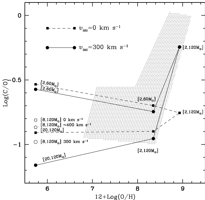
Fig. 20. Simplified model for the galactic evolution of the C/O ratio as a function of the O/H ratio (in number). The dashed and continuous lines show the results deduced from the non-rotating and the rotating models respectively (see text). The range of the initial masses used for computing the integrated yields are indicated. The empty symbols show the results when only stars more massive than 8 M_{\odot} are considered. The initial velocity is indicated. The shaded area shows the region where most of the observations of extragalactic HII regions and stars are located (see e.g. Gustafsson et al 1999; Henry et al. 2000).
