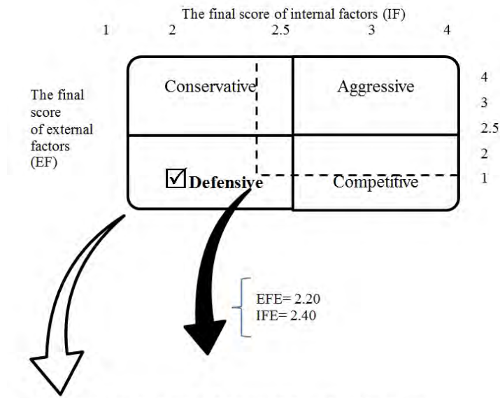
Fig. 3: Current status of environmental management in the area internal and external matrix (IE)
