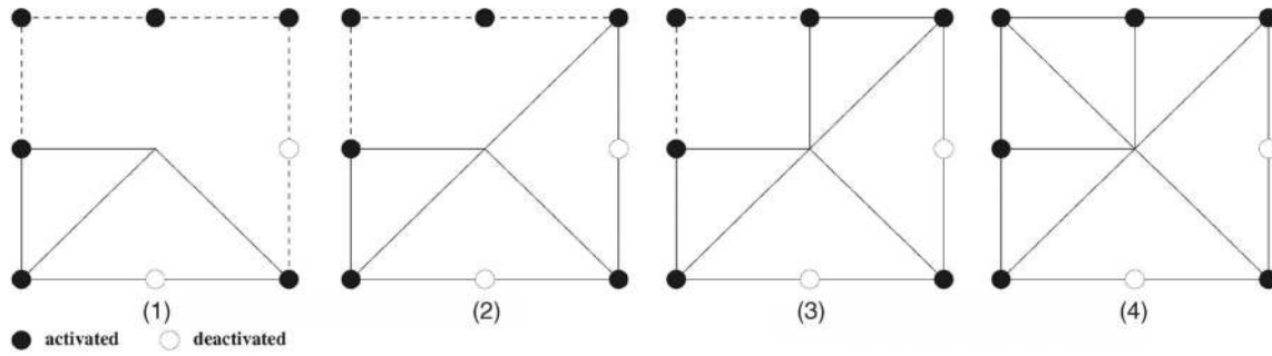
Fig. 7. A sample execution of the triangulation algorithm for a quad block.
