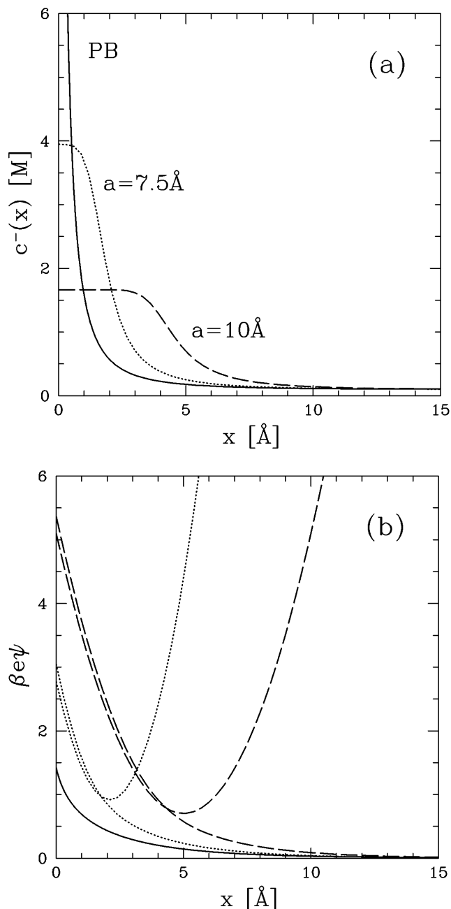
FIG. 1. (a) Concentration profiles of negative multivalent ions c^-(x) near a positively charged surface as obtained from the numerical solution of Eq. (3) for two different ion sizes a = 7.5 \text{ \AA} and a = 10 \text{ \AA} . Note that the saturated layer width is l^* \approx 2 and 5 \text{ \AA} , respectively. The solid line represents the concentration profile of the standard PB equation. (b) Calculated electrostatic potential profiles near the surface plotted together with the parabolic approximation [Eqs. (6) and (7)]. The dotted, dashed, and solid lines are as in (a). The bulk concentration is c_b = 0.1 \text{ M} for a 1:z electrolyte with z = 4 . The surface charge density \sigma is taken as one electron charge per 50 \text{ \AA}^2 . The aqueous solution with \epsilon = 80 is at room temperature.
