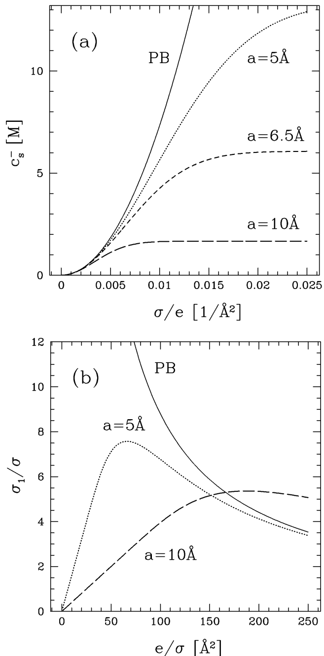
FIG. 2. (a) Surface concentration of ions as a function of the surface charge density for different ions size, a . The PB concentration is also plotted for comparison. (b) Ratio of the first layer charge density and the surface charge density, \sigma_1/\sigma = zec_s^- a/\sigma , as a function of the specific surface area per unit charge, e/\sigma , for different ion sizes. The PB result is plotted with the first layer width taken as 5 \text{\AA} . The 1:z electrolyte bulk concentration is c_b = 1 \text{ mM} and the valency z = 4 .
