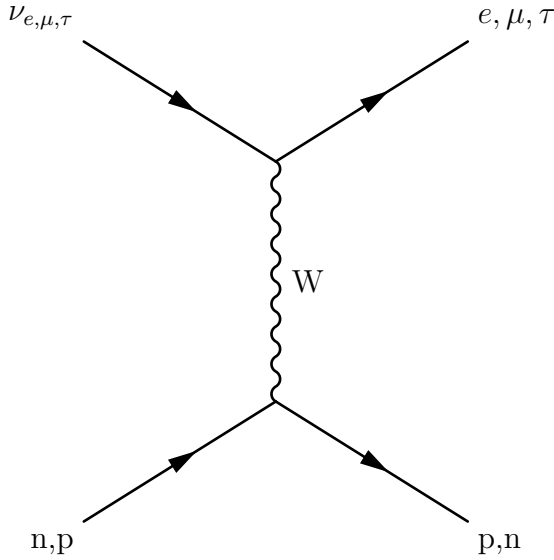
FIG. 4.1: Feynman diagram for a neutrino charged-current interaction. Where time goes from left to right.
