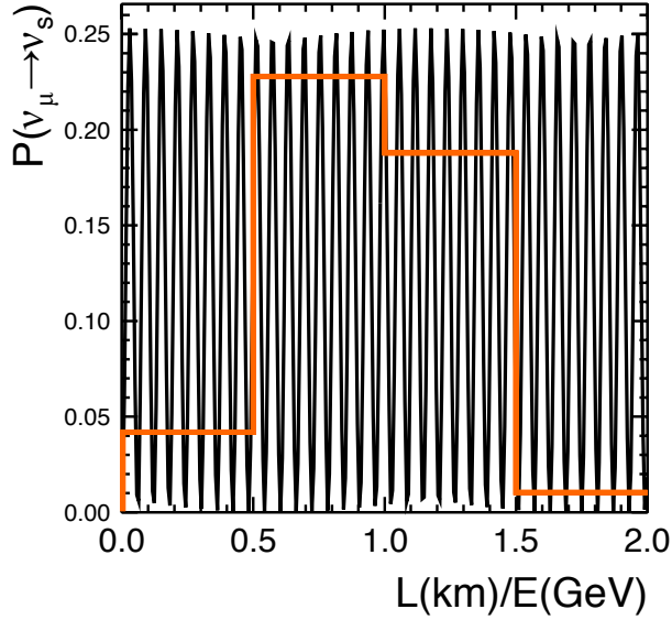
FIG. 5.15: The black curve represents the four flavor probability for \nu_\mu \rightarrow \nu_s at \Delta m_{34}^2 = 40.99\text{eV}^2 at the far detector baseline. The orange curve represents the calculated oscillation based on bin center.
