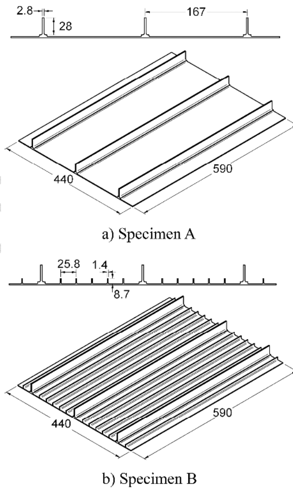
Fig. 2. Test specimen geometry.
