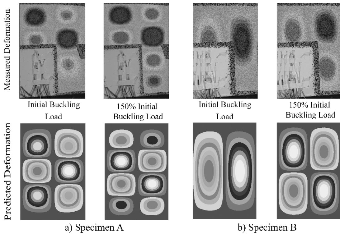
Fig. 4. Experimental and predicted out-of-plane deformations for Specimen A and Specimen B central skin bays.
