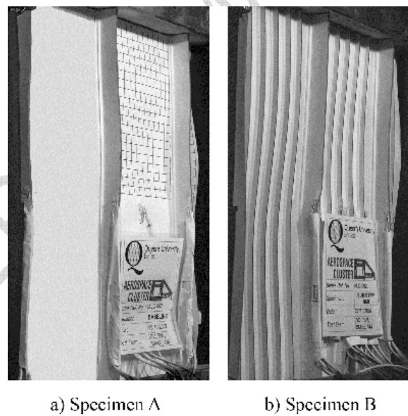
Fig. 5. Specimen collapse modes.
