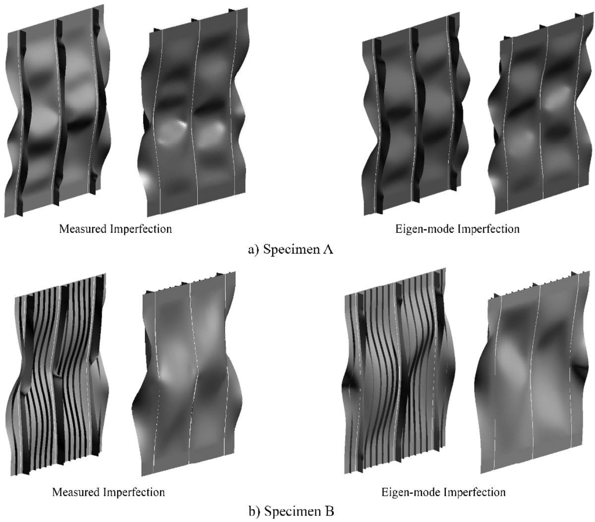
Fig. 8. Specimen simulation predicted collapse modes.
