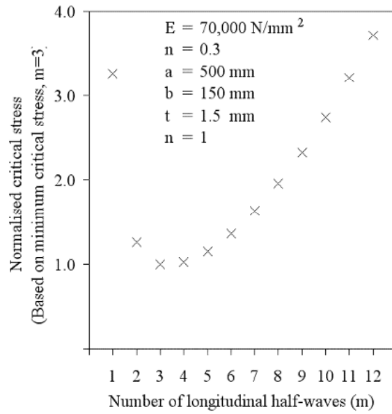
Fig. 1. Normalised compressive buckling stress for a flat rectangular plate simply supported on all edges.
