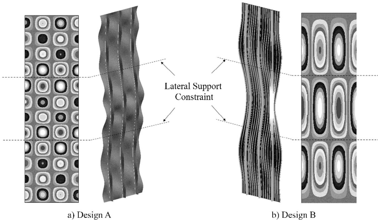
Fig. 10. Recurring panel models predicted initial buckling out-of-plane deformations and final collapse modes.
