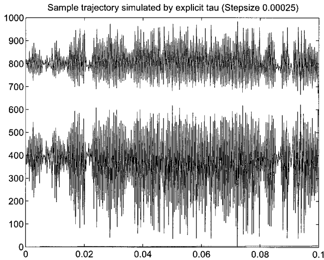
FIG. 6. Sample trajectories for example 1 as simulated by the explicit-tau method with step size 2.5 \times 10^{-4} . The trajectories develop unstable oscillations, and yield unrealistic negative states beyond t \approx 0.1 .
