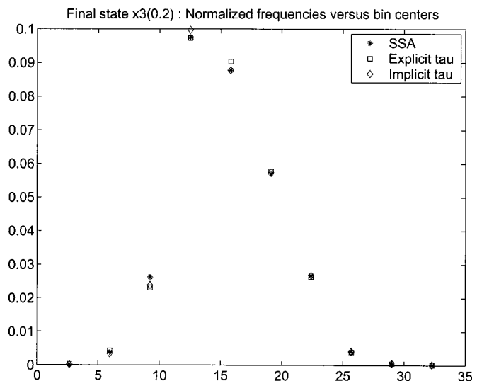
FIG. 9. Final state histogram for x_3 in example 1, as computed by the SSA (stars), the explicit-tau method with step size 1 \times 10^{-4} (squares), and the implicit-tau method with step size 0.01 (diamonds).
