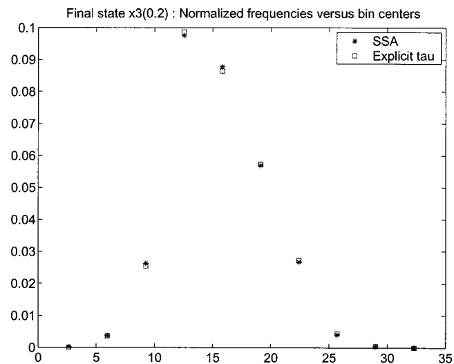
FIG. 5. Final state histogram for x_3 in example 1, computed by the SSA (stars) and the explicit-tau method (squares), the latter with constant step size 2 \times 10^{-5} .
