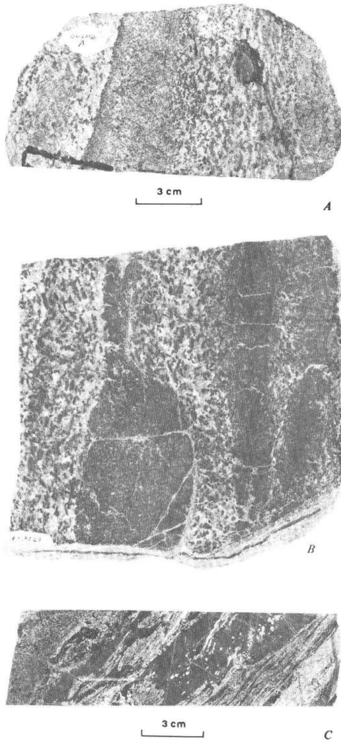
FIGURE 11.—Examples of compositional layering in metasedimentary rocks. A , Weathered surface. Dark minerals are orthopyroxene and minor biotite. Light minerals are quartz, cordierite, and minor plagioclase. B , Sawed slab. Black mineral is orthopyroxene; dark-gray mineral is cordierite; light-gray to white minerals are plagioclase and quartz. Slab is 18 cm wide. C , Hydrofluoric acid etched slab. Dark minerals are orthopyroxene and cordierite; light minerals are plagioclase and quartz.
