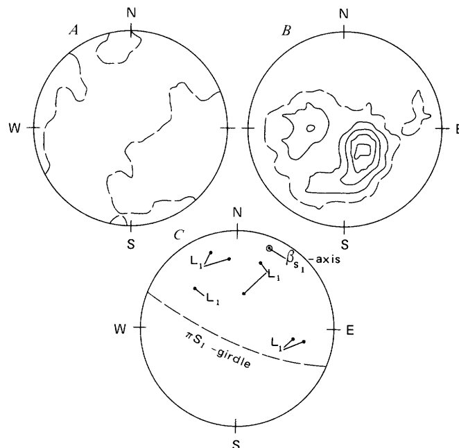
FIGURE 30.—Fabric diagrams of granitic gneisses and associated rocks in structural subareas 1 and 2. Contoured at 1E intervals where E is the expected number of points within the counting area for a random pattern using a method developed by Kamb (1959) and computerized by C. E. Corbató (written commun., 1970). Dashed contour is the 1E contour; solid contours are contours greater than 1E. A, Contoured poles to S_1 for subarea 1, 15 points, counting area=0.211, E=3.16 . B, Contoured poles to S_1 for subarea 2, 115 points, counting area=0.034, E=3.87 . C, L_1 fold axes and postulated \pi S_1 -girdle and \beta_{S_1} axis for subareas 1 and 2.
