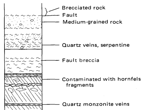
FIGURE 22.—Schematic diagrams of drill core showing contact relations between the coarse-grained quartz monzonite and the Basal norite member.
