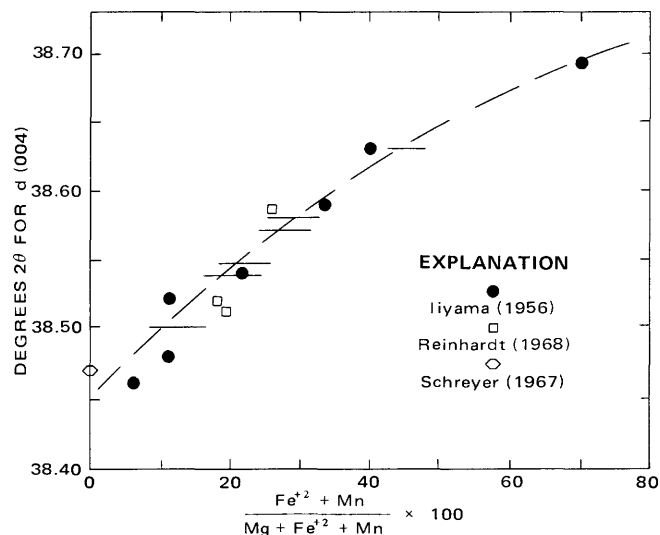
FIGURE 13.—X-ray determinative curve for (\text{Fe}^{2+} + \text{Mn}) / (\text{Mg} + \text{Fe}^{2+} + \text{Mn}) \times 100 ratio of cordierite. Horizontal lines indicate possible ratios for individual specimens of cordierite from the Stillwater Complex.
