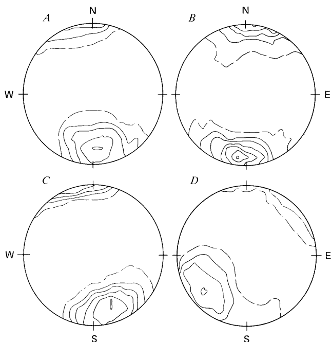
FIGURE 51.—Fabric diagrams of contoured poles to foliation for structural subareas of quartz monzonite. A, Medium-grained quartz monzonite, subarea 20, 22 points, counting area=0.154, E=3.38. B, Coarse-grained quartz monzonite, subarea 19, 67 points, counting area=0.056, E=3.77. C, Subarea 22, Granite Ridge area, 27 points, counting area=0.129, E=3.48. D, Subarea 21, 22 points, counting area=0.154, E=3.38. See figure 30 for explanation.
