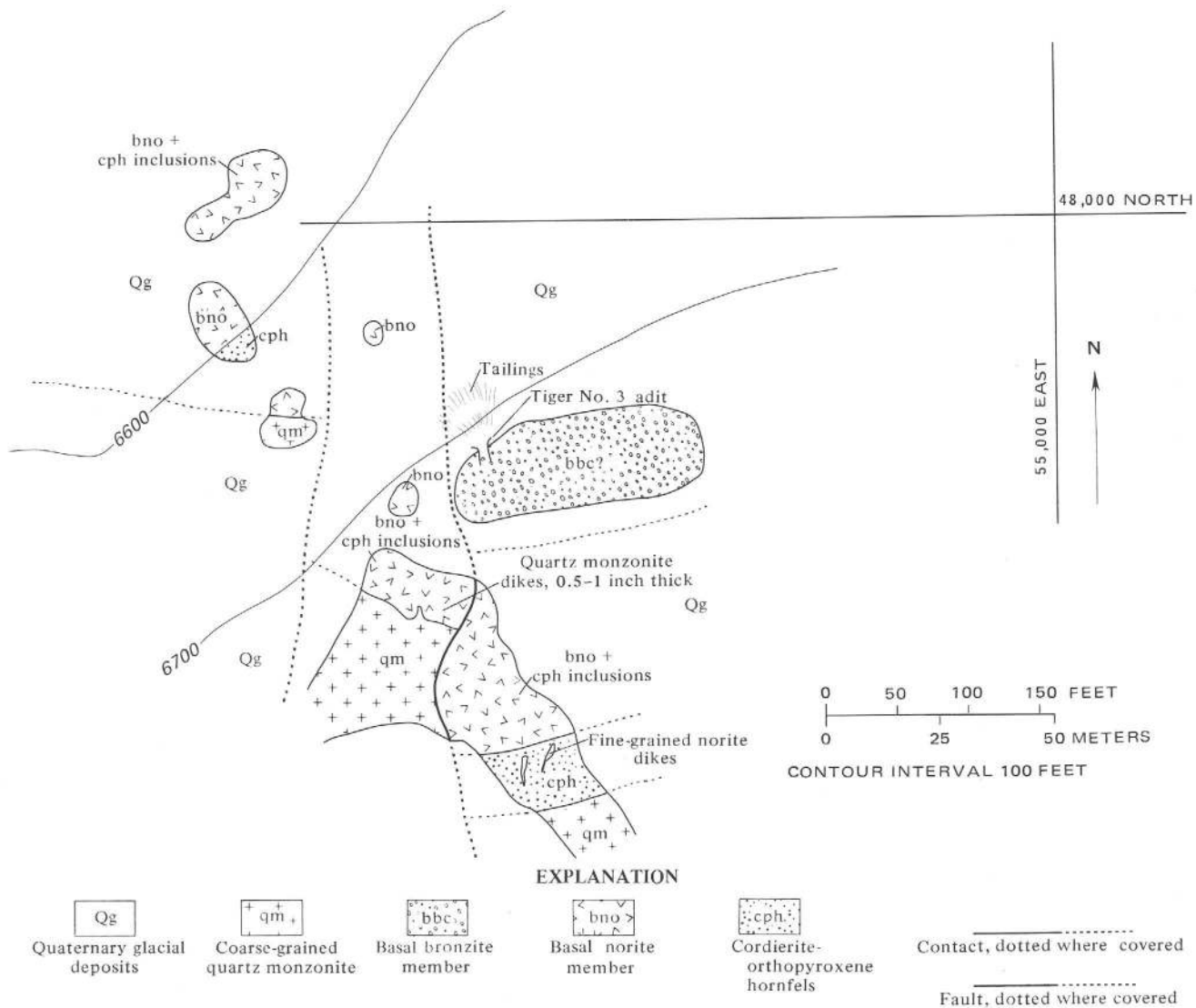
FIGURE 20.—Geologic sketch map of part of the Nye Lip area showing intrusive relations of the coarse-grained quartz monzonite. (Modified from Jackson and others, 1954; coordinates are those used by Jackson and others, 1954, in the Nye Lip area.)
