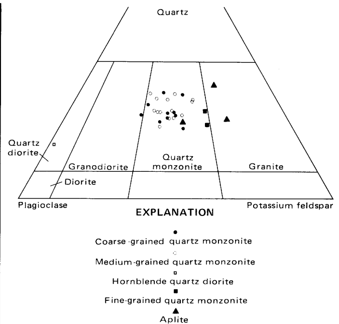
FIGURE 23.—Triangular diagram of modal quartz, plagioclase, and potassium feldspar in granitic intrusive rocks. Compositional names and subdivisions after Bateman, Clark, Huber, Moore, and Rinehart (1963).
