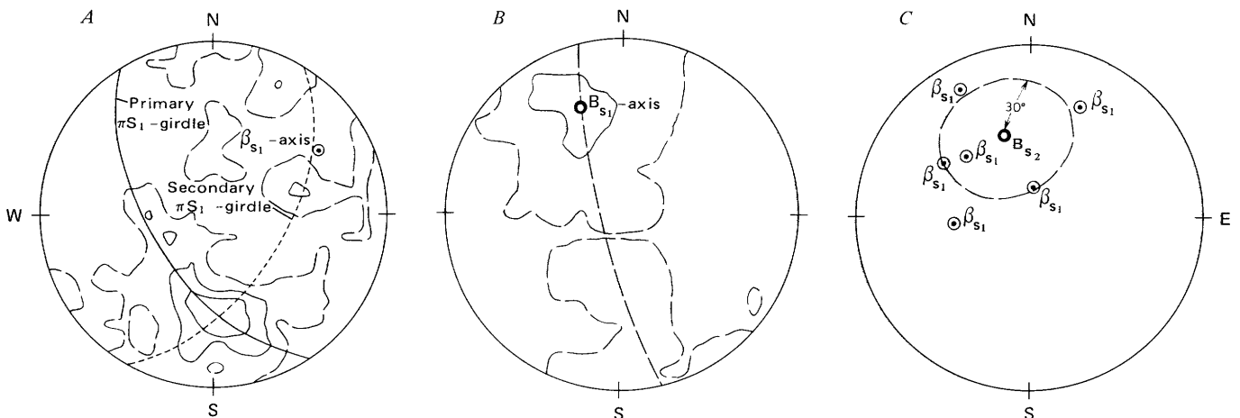
FIGURE 45.—Contoured fabric diagrams of all structures in structural subareas (1, 2, 4, 5, 6) exclusive of the Mountain View area (subarea 3). A, Poles to layering ( S_1 ), 263 points, counting area=0.015, E=3.94 ; see figure 30 for explanation. B, L poles, 18 points, counting area=0.182, E=3.27 . Long-dashed line, weak girdle formed by fold axes (L). C, Plot of \beta_{S_1} poles from all subareas (1-6) and parts of subareas. Dashed circle formed by \beta_{S_1} axes from each subarea. \beta_{S_2} fold axes from Mountain View area (fig. 36A).
