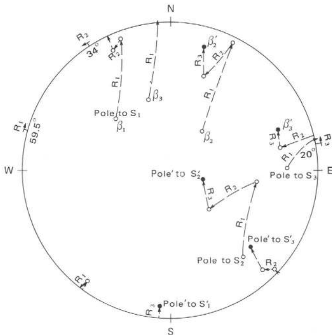
FIGURE 56.—Rotation of attitudes of cumulus layering ( S_1 ), axial planar cleavage ( S_2 ), cleavage ( S_3 ), and fold axes ( \beta S_1 ) and \beta S_2 ) in hornfels in the Mountain View area to their position at the time of intrusion of the Stillwater Complex. Rotation axes: R_1 N. 298.5° E., 59.5° counterclockwise to south; R_2 , N. 327° E., 34° clockwise to north; R_3 , N. 80° E., 20° clockwise to south.
