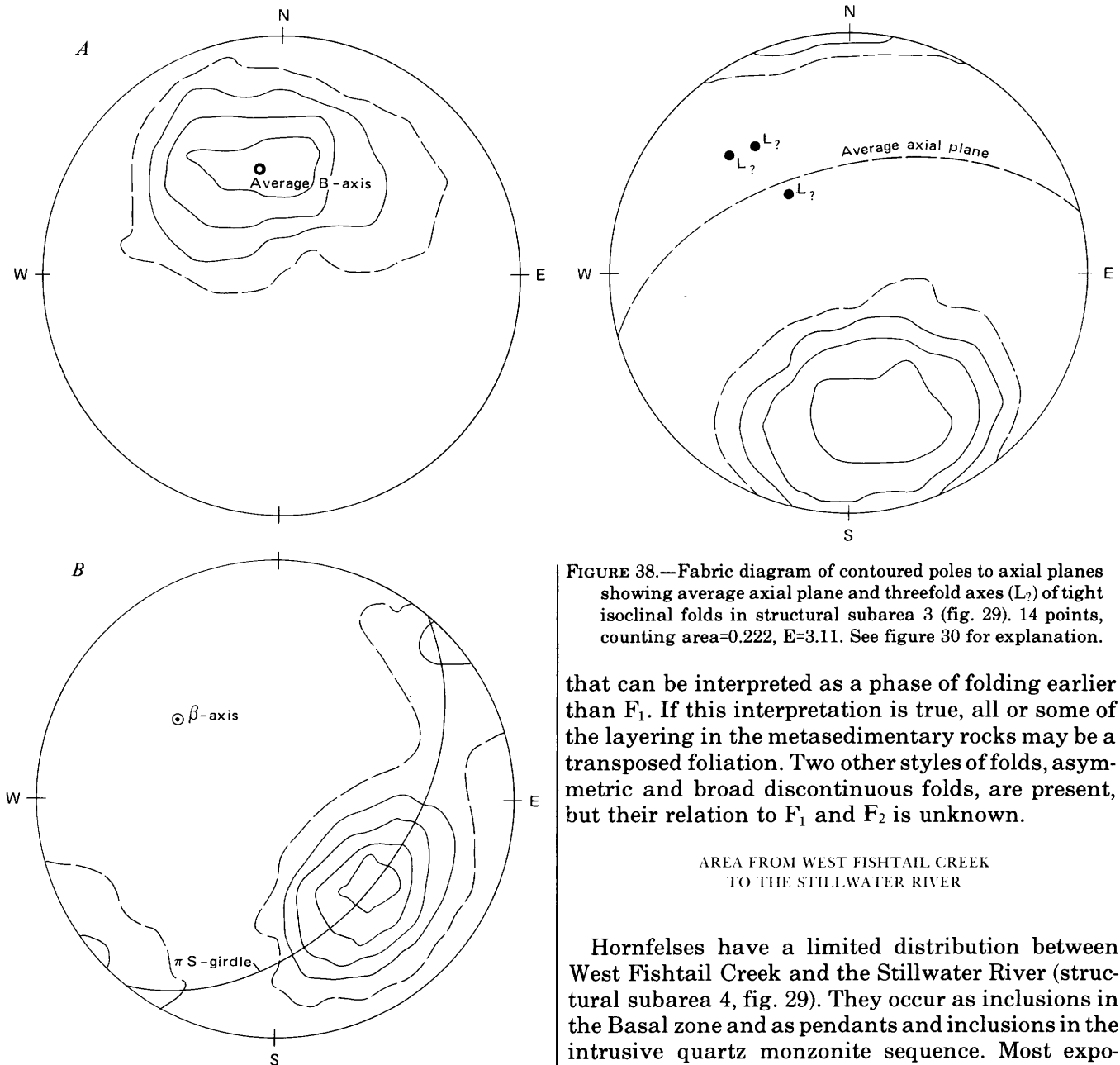
FIGURE 37.—Contoured fabric diagrams of fold axes ( L_2 ) and axial planes ( S_2 ) of discontinuous broad folds and asymmetric folds. A, L_2 , 28 points, counting area=0.125, E=3.50. B, Poles to S_2 , 55 points, counting area=0.068, E=3.73. See figure 30 for explanation.
