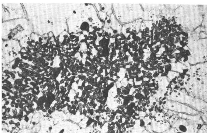
FIGURE 14.—Photomicrographs of thin sections showing hornfels textures. Black minerals, magnetite and sulfide; dark-gray mineral, spinel; medium-gray high-relief mineral, orthopyroxene; white to light-gray mineral, cordierite. Partly crossed nicols. A , Euhedral spinel with cordierite. Spinel grains 0.2 mm wide. B , Clots of fine spinel in cordierite. Width of B , 1 mm. Photographs by N. F. Prime.
