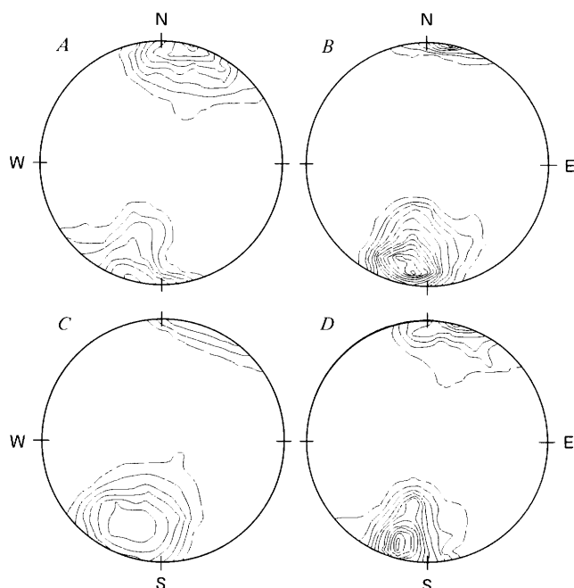
FIGURE 50.—Fabric diagrams of contoured poles to igneous layering ( S_0 ) in the Banded and Upper zones of the Stillwater Complex. See figure 30 for explanation. A, Structural subarea 18, 118 points, counting area=0.033, E=3.87 . B, Structural subarea 17, 98 points, counting area=0.039, E=3.84 . C, Structural subareas 15 and 16, 27 points, counting area=0.129, E=3.48 . D, All subareas combined, 243 points, counting area=0.016, E=3.94 .
