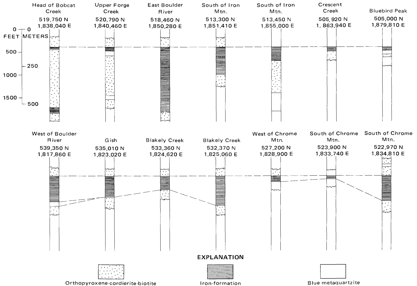
FIGURE 8.—Reconstructed partial columns for the iron-formation between Bluebird Peak and the Boulder River. Coordinates are from near the contact of the iron-formation with other units. All sections constructed perpendicular to strike of units.
