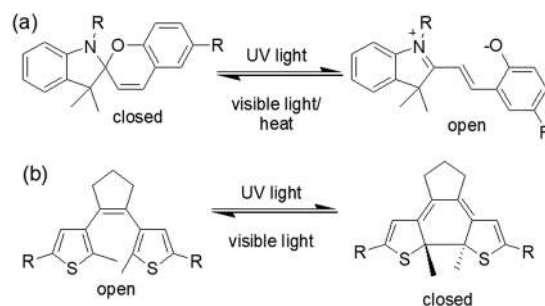
Fig. 9 Photoresponsive ring closing and opening of (a) spiroopyran and (b) dithienylethene molecules.
