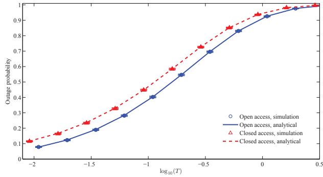
Fig. 7. Femtocell outage probability under different T , with \lambda = 8 units/km 2 /sub-band and \mu = 8 units/km 2 /sub-band.
