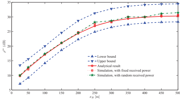
Fig. 10. \rho^{**} under different \mathbf{x}_B , \mathbf{x}_B = (x_B, 0) , at the femtocell level.
