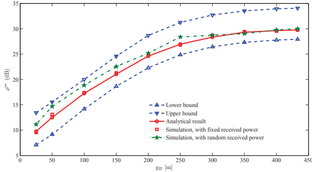
Fig. 11. \rho^{**} under different \mathbf{x}_B , \mathbf{x}_B = (0, y_B) , at the femtocell level.
