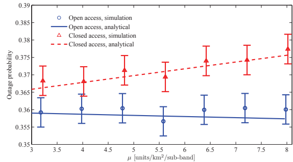
Fig. 4. Macrocell outage probability under different \mu , with \lambda = 4 units/km 2 /sub-band and T = 0.1 .
