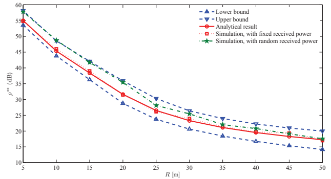
Fig. 9. \rho^{**} under different R at the femtocell level.
