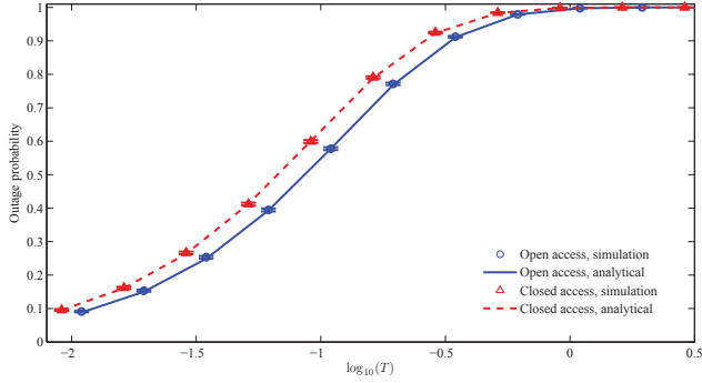
Fig. 6. Macrocell outage probability under different T , with \lambda = 8 units/km 2 /sub-band and \mu = 8 units/km 2 /sub-band.
