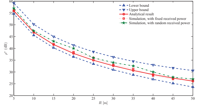
Fig. 8. \rho^* under different R at the macrocell level.
