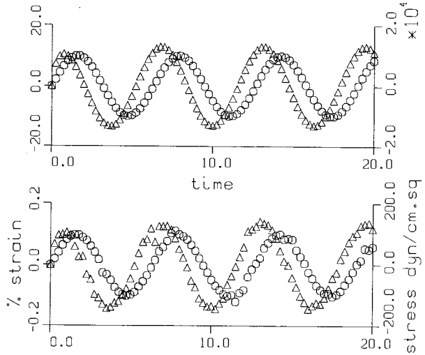
Figure 2.1: Strain and stress as function of time in an oscillatory shear flow, measured at a PS sample (Rheometrics): (a) Strain amplitude 10%; (b) Strain amplitude (0.1%), so that the experimental noise is high
