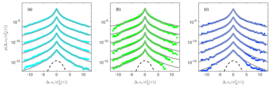
Figure 4. Probability distribution of velocity increments from normalized t-Lagrangian velocities (symbols) and their respective CTRW model simulations (gray lines) for samples (a) A, (b) B, and (c) C. Increments are determined at time lags of \tau = 0.05\tau_v, 0.1\tau_v, 0.33\tau_v, 0.5\tau_v, \tau_v , and 2\tau_v , arranged from top to bottom. Dashed black line is a reference Gaussian distribution.
