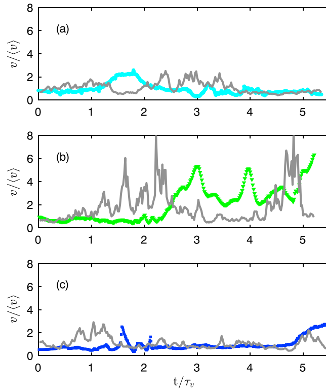
Figure 2. Symbols are time series of exemplary t-Lagrangian particle velocities for structures (a) A, (b) B, and (c) C. Gray lines correspond to simulated isochrone trajectories from the CTRW model.
