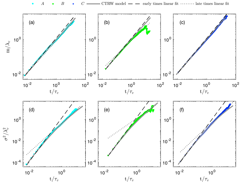
Figure 1. Symbols are (a–c) normalized mean displacement or (d–f) mean square displacement of tracer particles over normalized time for samples A (Figures 1a and 1d), B (Figures 1b and 1e), and C (Figures 1c and 1f). Dashed and dotted lines are the linear fits for the early and late times, respectively. Solid lines are predictions of the CTRW model.
