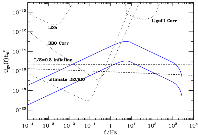
FIG. 1: Spectrum of GW background from Eq. (4) for a simulation from Ref. [7]. Solid lines: the spectrum is continuously extended with the low- f tail according to Eq. (3). The upper curve is obtained from Fig. 9 of Ref. [7], whereas the lower is the same shifted downwards by a factor 100, which is considered a more realistic estimate. Horizontal lines: GW stochastic spectrum produced during slow-roll inflation and evaluated from Eq. (6) of Ref. [17]. We assume T/S = 0.3 for the ratio of the tensorial and scalar contributions to the cosmic microwave background radiation (CMBR) anisotropy and consider two values \pm 10^{-3} of the running of the tensorial power-law index. Dotted lines: sensitivities of the indicated detectors. The BBO sensitivity is approximate and may change slightly in the final design.
