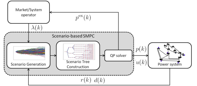
Fig. 1: Scenario-based SMPC for optimal power dispatch
