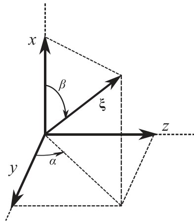
FIG. 13. Wave vector geometry of a single Fourier mode.
