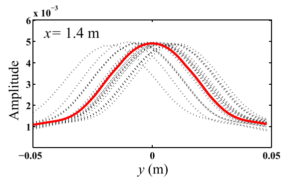
FIG. 21. Amplitude distributions along the line x=1.4\text{ m} calculated by the stochastic model; the solid (red) curve denotes the result in a mean homogeneous medium and the dotted curves denotes the results in the random medium, mean deviation: \sim 10\text{ mm} , standard deviation of gaps: 7.6\text{ mm} .
