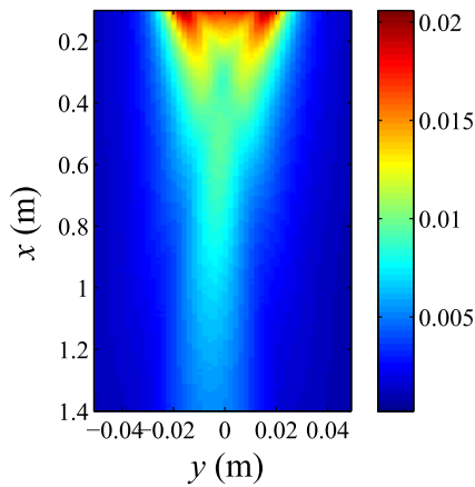
FIG. 18. Acoustic beam propagation in a inhomogeneous medium calculated by the deterministic ray tracing model.
