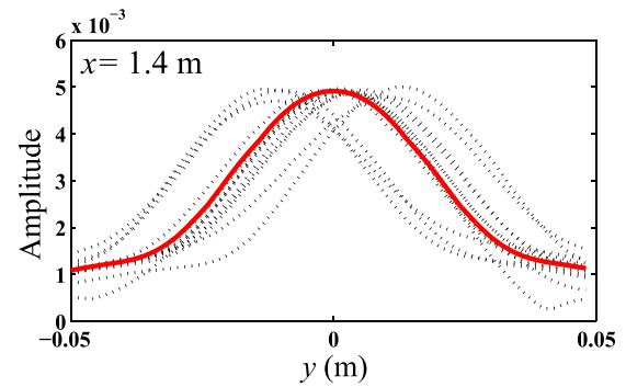
FIG. 20. Amplitude distributions along the line x=1.4\text{ m} calculated by the deterministic model; the solid (red) curve denotes the result in a mean homogeneous medium and the dotted curves denotes the results in the random medium, mean deviation: \sim 10\text{ mm} , standard deviation of gaps: 7.3\text{ mm} .
