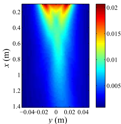
FIG. 19. Acoustic beam propagation in a inhomogeneous medium calculated by the stochastic simulation model.
