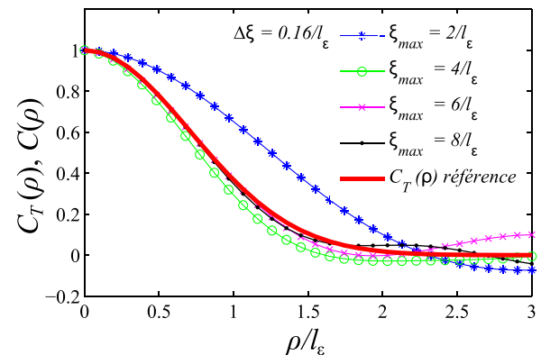
FIG. 11. Comparison between the theoretical (red line) and simulated covariance functions obtained for \xi_{\max} = 2/l_\epsilon (blue), 4/l_\epsilon (green), 6/l_\epsilon (purple), 8/l_\epsilon (black), and \Delta\xi = 0.16/l_\epsilon .
