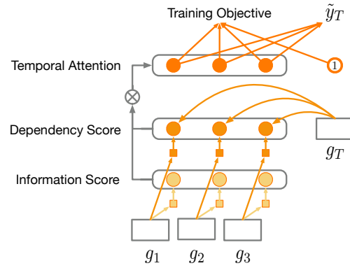
Figure 3: The temporal attention in our model. Squares are the non-linear projections of g_t and points are scores or normalized weights.
