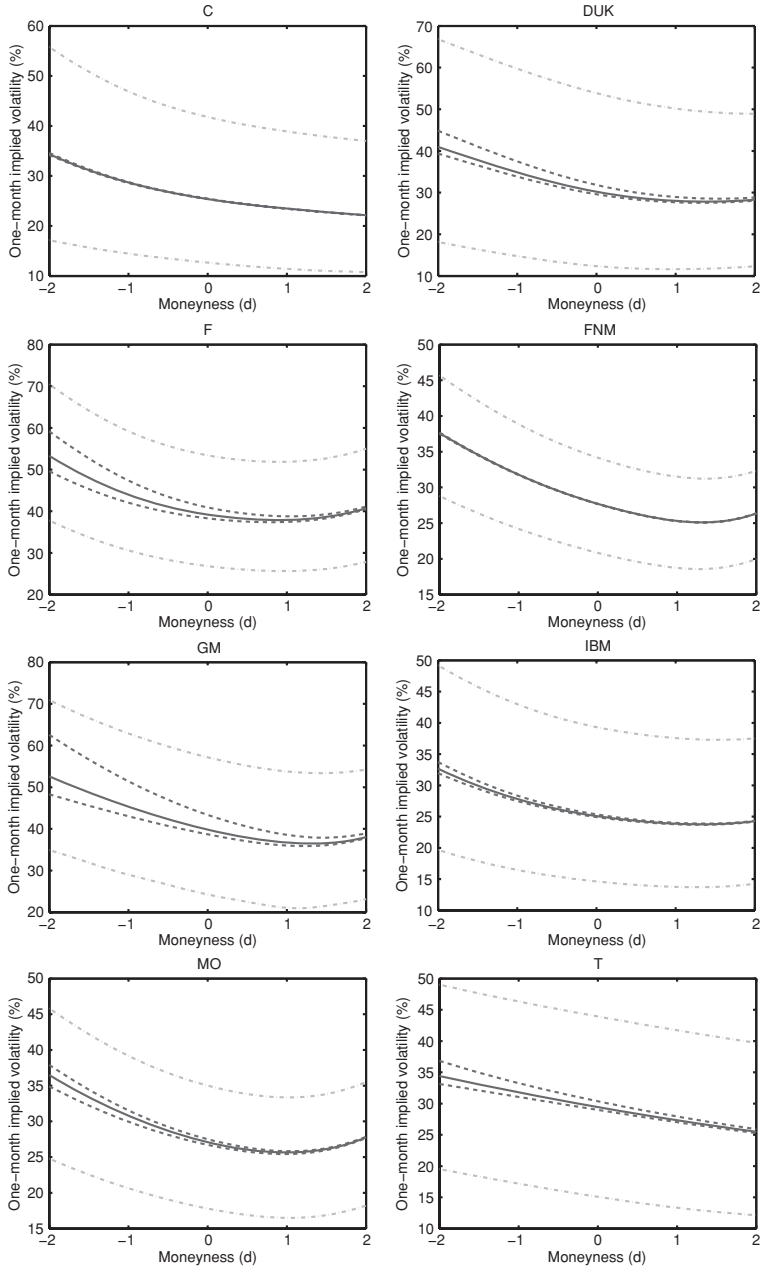
Figure 7 The one-month implied volatility smirks. The solid lines are the mean implied volatility across moneyness at one-month maturity computed from the estimated model and the sample mean levels of the two risk factors. Moneyness is defined as d = \ln(K/S)/\sqrt{v\tau} . Dashed lines are computed by setting v_t to its sample average and z_t to its 10th and 90th percentile values. Dash-dotted lines are computed by setting z_t to the sample mean and v_t to its 10th and 90th percentile values.
