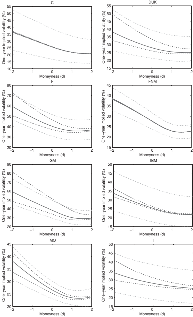
Figure 8 The one-year implied volatility skews. The solid lines are the mean implied volatility computed across moneyness at one-year maturity from the estimated model and the sample mean levels of the two risk factors. Moneyness is defined as d = \ln(K/S)/\sqrt{v\tau} . Dashed lines are computed by setting v_t to its sample average and z_t to its 10th and 90th percentile values. Dash-dotted lines are computed by setting z_t to the sample mean and v_t to its 10th and 90th percentile values.
