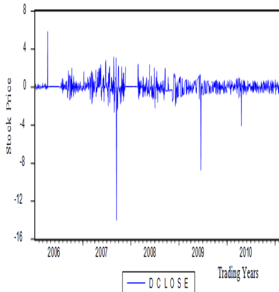
Figure 10: Graphical representation of the Zenith bank stock index first differencing
