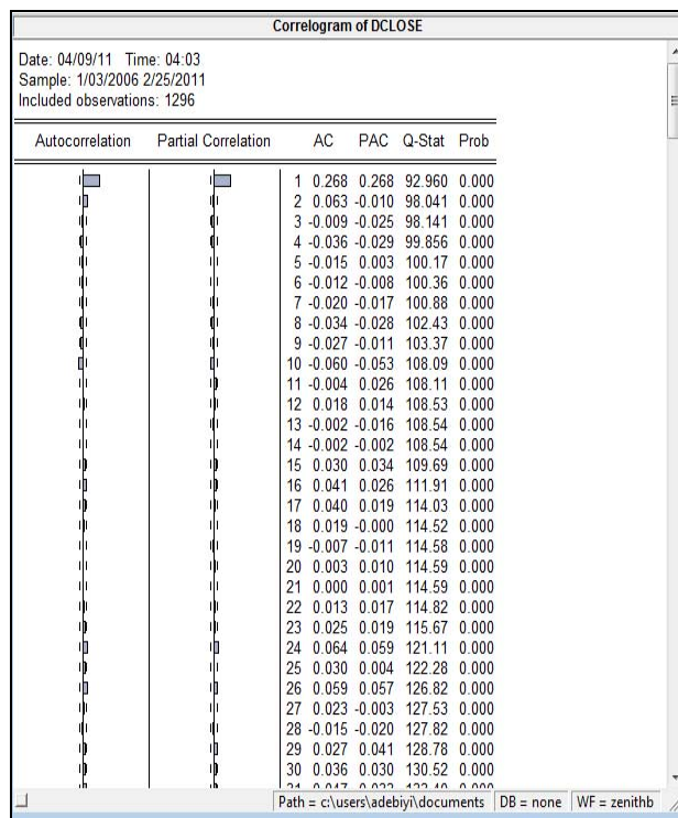
Figure 11: The correlogram of Zenith bank stock price index after first differencing.
