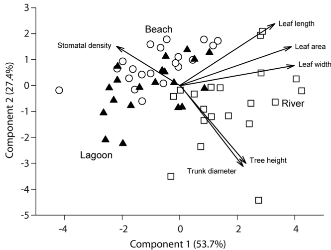
Fig. 4. Biplot indicating the distribution of the scores from the Principal Component Analysis and the variables used for Rhizophora mangle tree and leaf characterization in three sampling sites (River, squares; Lagoon, triangles; Beach, circles) within the Xel-Há cove, Quintana Roo, Mexico. Each data point represents a tree.
