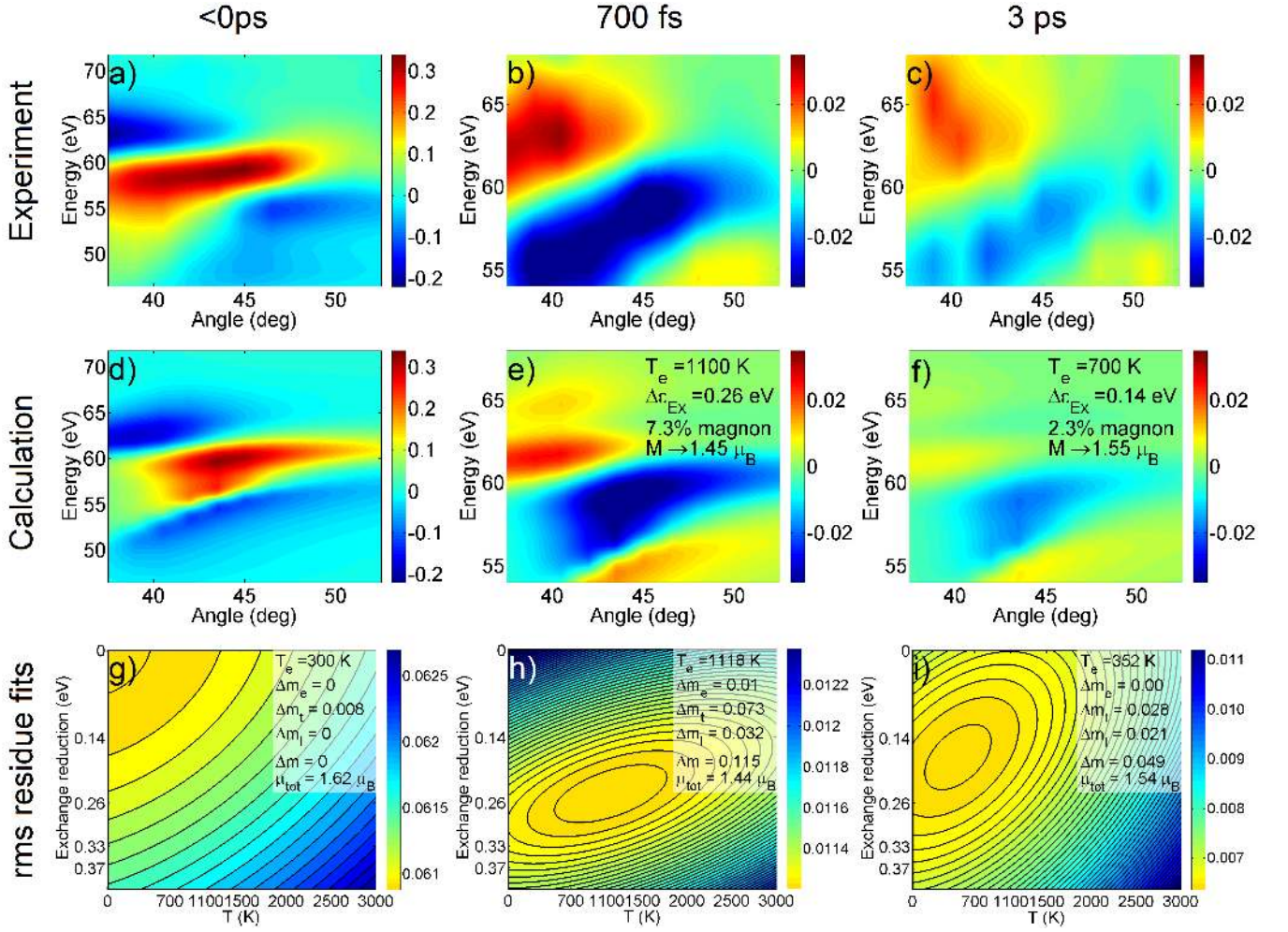
FIG. 3. Comparison of the experimental (a) and theoretical (d) angle- and energy-resolved T-MOKE asymmetries before laser excitation. Comparison of the experimental (b, c) and theoretical (e, f) differential asymmetry spectra at 0.7 ps and 3 ps. The measured differential spectra (b) and (c) at both delay-times exhibit distinct qualitative differences from the spectrum at time-zero, (a). (e) and (f) show specific examples of calculated spectra near the optimal values determined from the least-squares-fit. Last row (g)-(i) - contour plots of quadratic fits to rms residues resulting from independent fitting of ab initio calculated spectra to measured spectra. It can be clearly seen how the Co film is excited by a femtosecond laser pulse from <math><0\text{ps}</math> (g) to 0.7 ps (h) and how it relaxes back towards equilibrium from 0.7 ps (h) to 3 ps (i). In (g) \Delta m_t = 0.008 is based on Ref. 42 .
