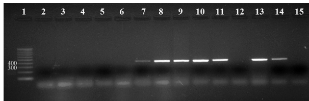
Agarose gel showing amplifications of polymerase chain reaction of Giardia intestinalis which were stored six different conditions. Lane 1: 100 bp Plus DNA Ladder (Vivantis); 2-7: sample contain more Giardia trophozoites than Giardia cyst; 8-13: sample contain only Giardia cyst; 2, 8: from sample stored at room temperature; 3, 9: from sample stored at +4°C; 4, 10: from sample stored at -20°C; 5, 11: from sample stored at 70% alcohol; 6, 12: from sample stored at 10% formaldehyde; 7, 13: from sample stored at 2.5% potassium dichromate; 14: positive control; 15: negative control.
