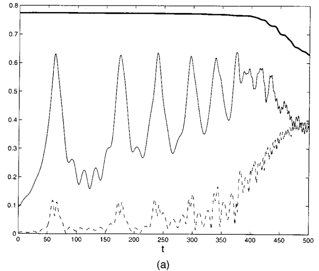
Fig. 16. (Experiment 2.2a) Capture of a gap soliton with \delta = 0.45 by a wide well.
