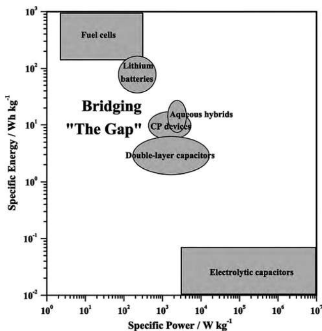
Fig. 15 Ragone plot illustrates different types of energy-storage devices as a function of specific power and energy. Reprinted from ref. 78 with permission from Elsevier.
