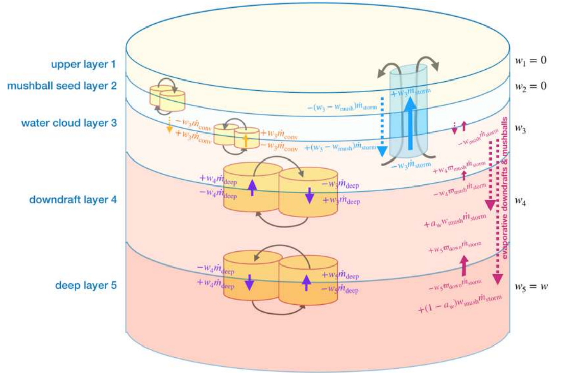
Figure 3. As Figure 2 for the mass balance of water in the framework of our five-layer model. Compared to Figure 2, the main differences arise from the fact that water precipitates out of layers 2 and 1 so that its abundance in these layers is, on average, extremely small. Also, the evaporation of mushballs removes a fraction a_w of the water which is incorporated into layer 4, with the remaining 1-a_w being incorporated into layer 5.
