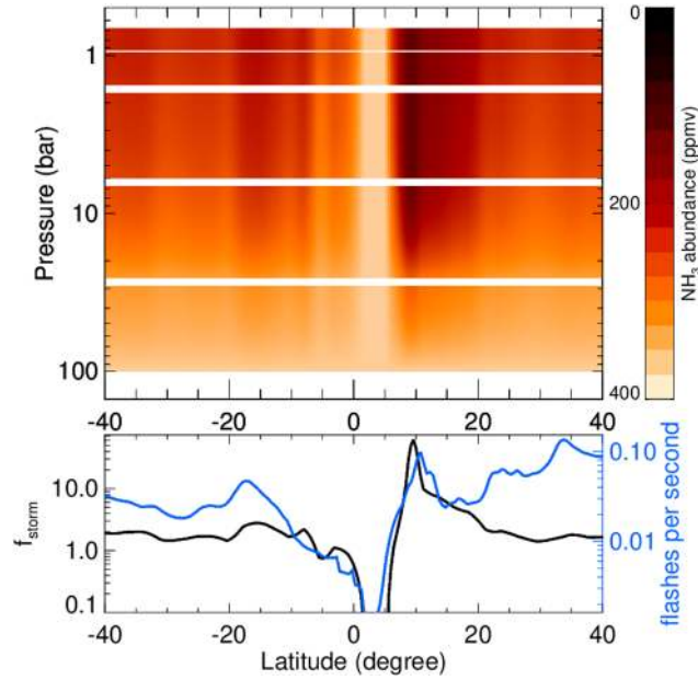
Figure 6. Distribution of ammonia concentration obtained with our mass balance model. The top panel shows the \text{NH}_3 mixing ratio as a function of latitude and pressure in the five layers of our model. The bottom panel indicates the value of f_{\text{storm}} (black line) obtained to reproduce the 1- to 3-bar MWR ammonia mixing ratio compared to the number of flashes per second detected by the MWR instrument between PJ1 and PJ16 (Brown et al., 2018). The large and uniform ammonia concentration in the Equatorial Zone is well reproduced by assuming a scarcity of storms ( f_{\text{storm}} \sim 0 ), in line with the absence of lightning there. At middle latitudes, frequent storms and subsequent mushball formation lead to a depletion of ammonia.
