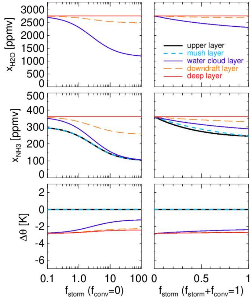
Figure 5. Abundances of water (top row), ammonia (middle row), and potential-temperature anomalies (bottom row) obtained with our model, as a function of f_{\text{storm}} , a parameter assessing the mass flux in large water storms relative to that of dry convection below the water cloud base. The left column corresponds to a situation in which no small-scale convection is present in the water condensation region ( f_{\text{conv}} = 0 ) and pertains to midlatitude regions of Jupiter. The right column assumes that both small-scale convection and storms occur, so that f_{\text{storm}} + f_{\text{conv}} = 1 . The curves show the different layers considered in Figure 5: (1) upper layer (purple); (2) mushball-seed layer (blue, dashed); (3) water cloud layer (light blue); (4) downdraft layer (orange, dashed); and (5) deep (red). The potential-temperature anomalies are calculated assuming that intrinsic heat flux transport occurs with negligible superadiabicity (see text).
