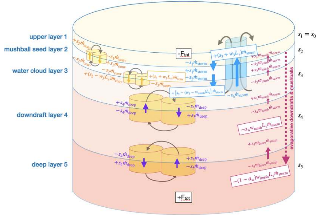
Figure 4. As Figure 2 for the balance of static energy in the framework of our five-layer model. In addition to the terms due to a transport of static energy, terms resulting from the condensation or evaporation of water are highlighted. A flux F_{\text{tot}} arising from internal heat is added to layer 5 and removed from layer 1.
