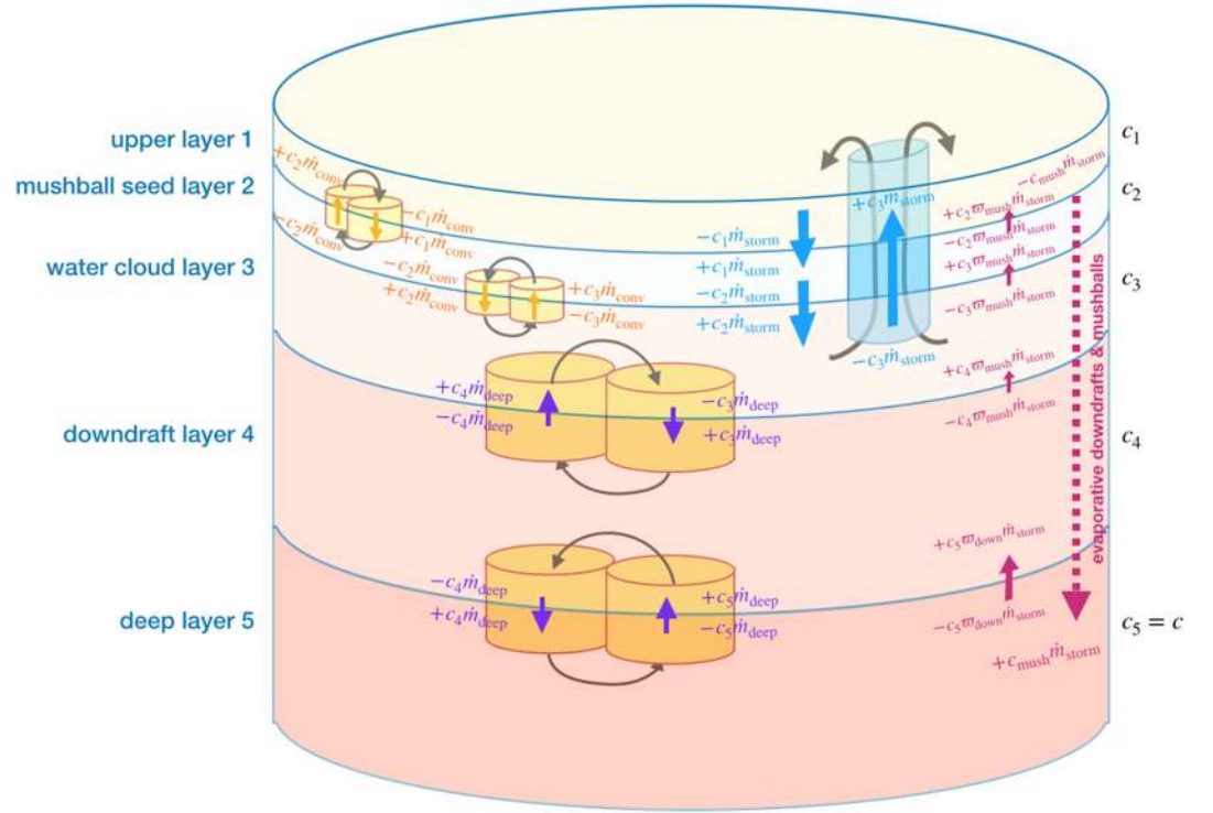
Figure 2. Mass balance of ammonia in the framework of our five-layer model. We consider that three main processes transport material between layers: In yellow, small-scale convection is modeled as an updraft and its reciprocal downdraft between adjacent layers. We consider that it is characterized by an upward mass flux \dot{m}_{\text{deep}} between layers 5 and 4 and layers 4 and 3, and by an upward mass flux \dot{m}_{\text{conv}} between layers 3 and 2 and layers 2 and 1. In blue, strong storms due to water condensation lead to a transport of material directly from layer 3 to layer 1 and to a compensating subsidence mass flux from layer 1 to layer 2 and to layer 3. These storms also lead to the formation of mushballs and evaporative downdrafts which deliver ammonia and water directly to layers 4 and 5. The terms in each layer correspond to the mass balance of ammonia described by equation.
