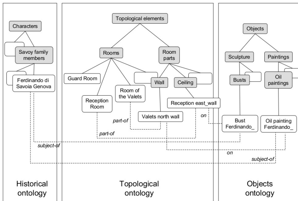
Figure 4. A fragment of the domain ontology concerning Palazzo Chiabilese, including portions of three ontologies (historical, topological and object ontologies). Grey boxes represent classes, white boxes represent instances. Subclass and instance relations are represented by solid lines, non-taxonomic relations are represented by dashed lines.
